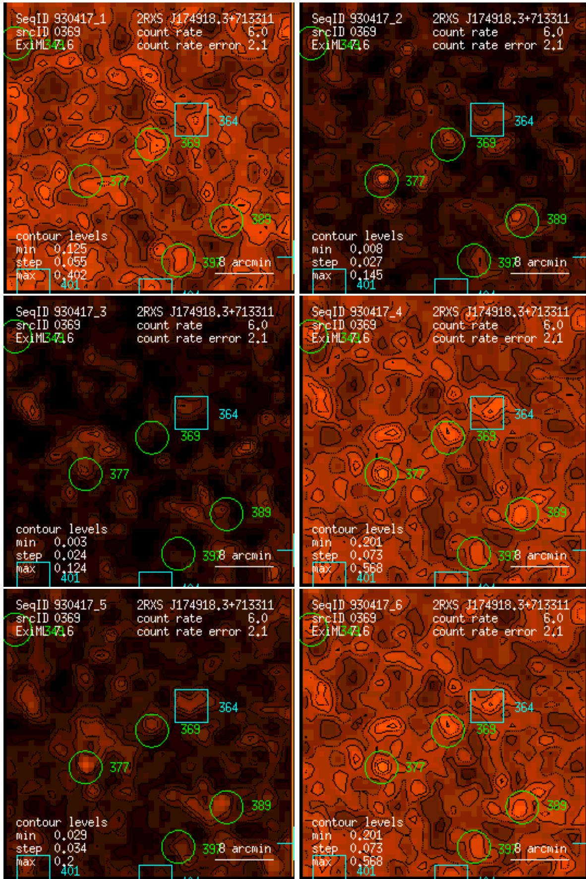
Figure 369: RASS 930417: detection 0369: band rate images, Gaussian filter: (1) PSPC channels 11 – 41, (2) 52 – 90, (3) 91 – 201, (4) 11 – 235, (5) 52 – 201, (6) 11 – 201. Broad band rates in counts/ks. Band rate contour levels in counts/ks/arcmin 2 .
