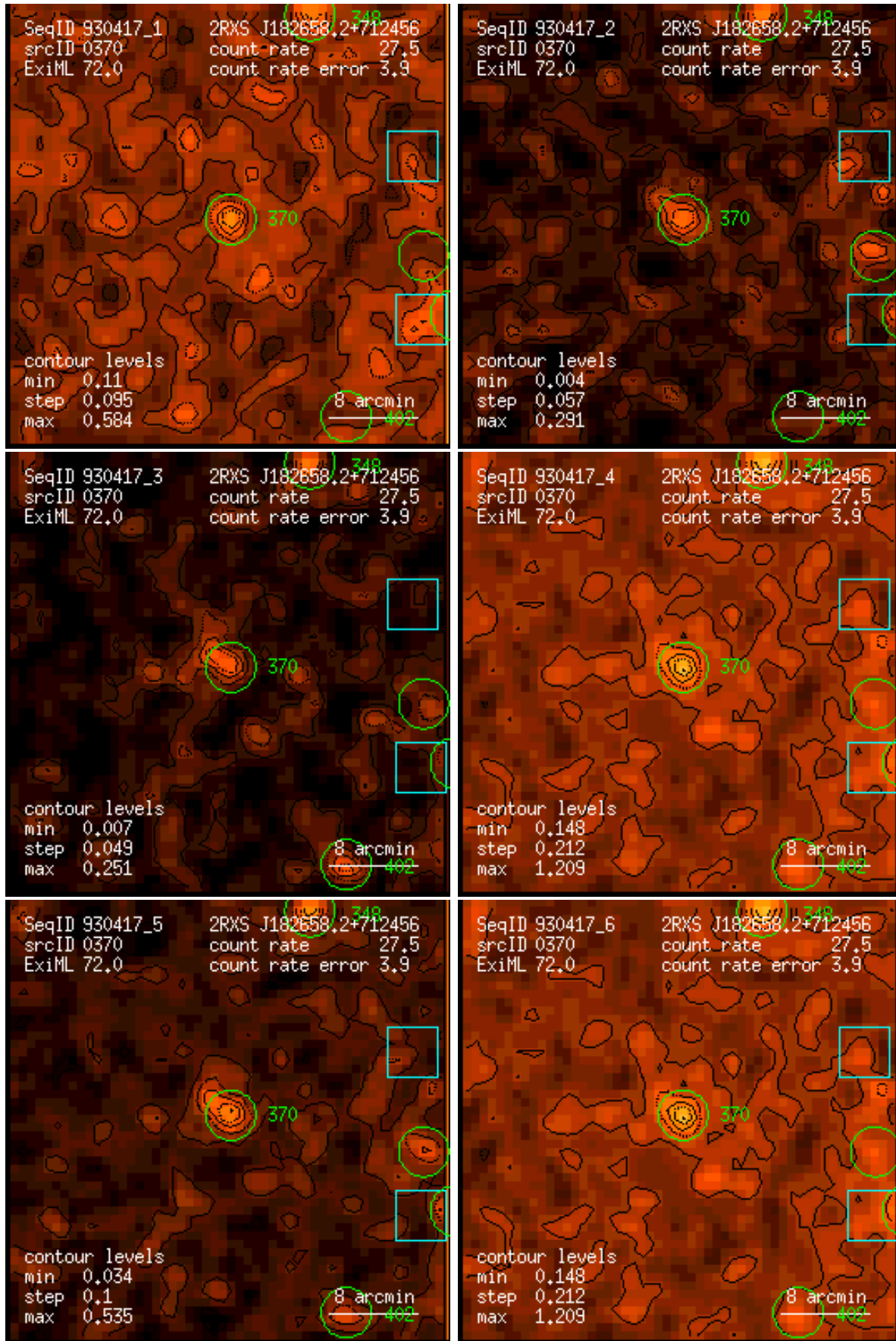
Figure 370: RASS 930417: detection 0370: band rate images, Gaussian filter: (1) PSPC channels 11 – 41, (2) 52 – 90, (3) 91 – 201, (4) 11 – 235, (5) 52 – 201, (6) 11 – 201. Broad band rates in counts/ks. Band rate contour levels in counts/ks/arcmin 2 .
