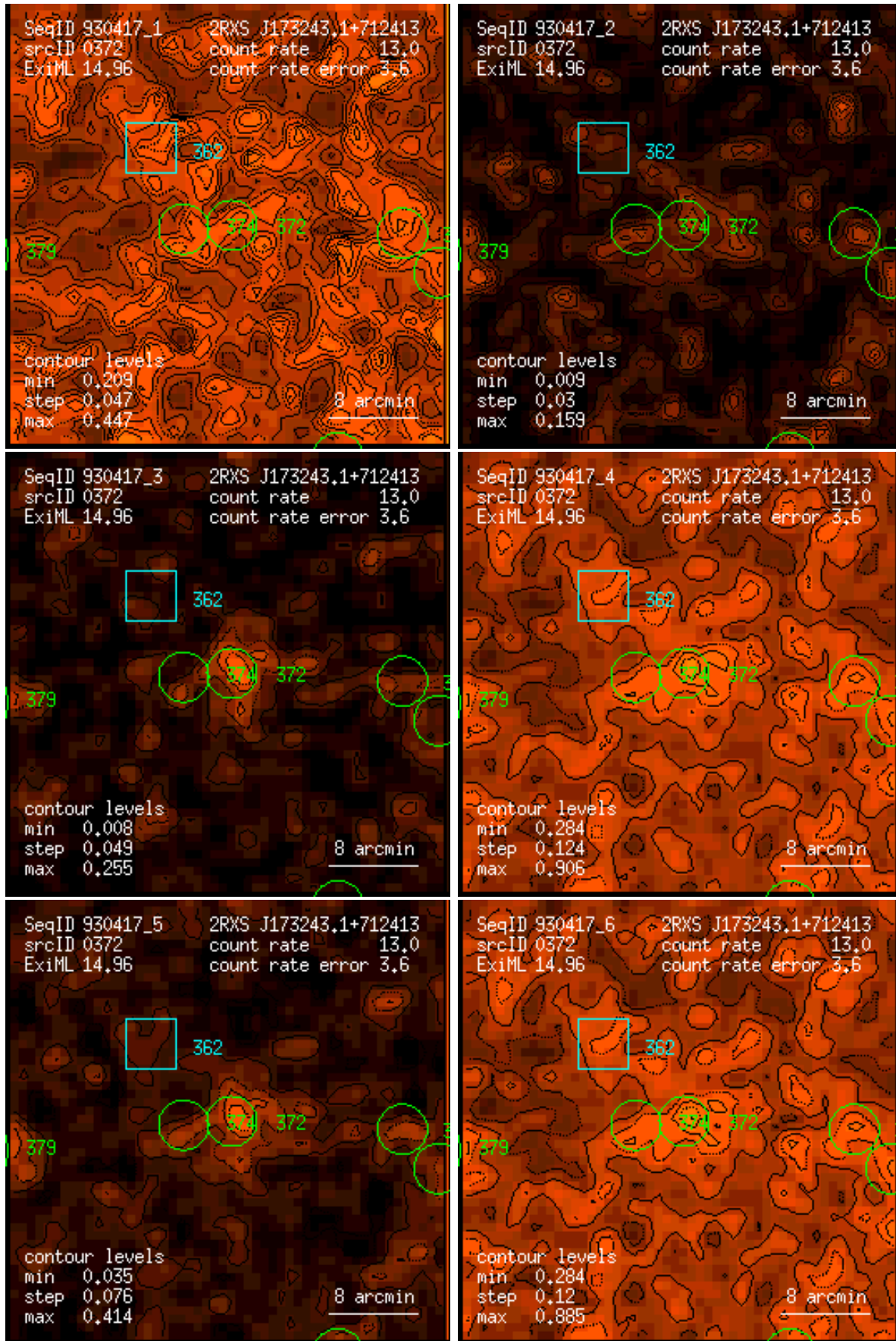
Figure 372: RASS 930417: detection 0372: band rate images, Gaussian filter: (1) PSPC channels 11 – 41, (2) 52 – 90, (3) 91 – 201, (4) 11 – 235, (5) 52 – 201, (6) 11 – 201. Broad band rates in counts/ks. Band rate contour levels in counts/ks/arcmin 2 .
