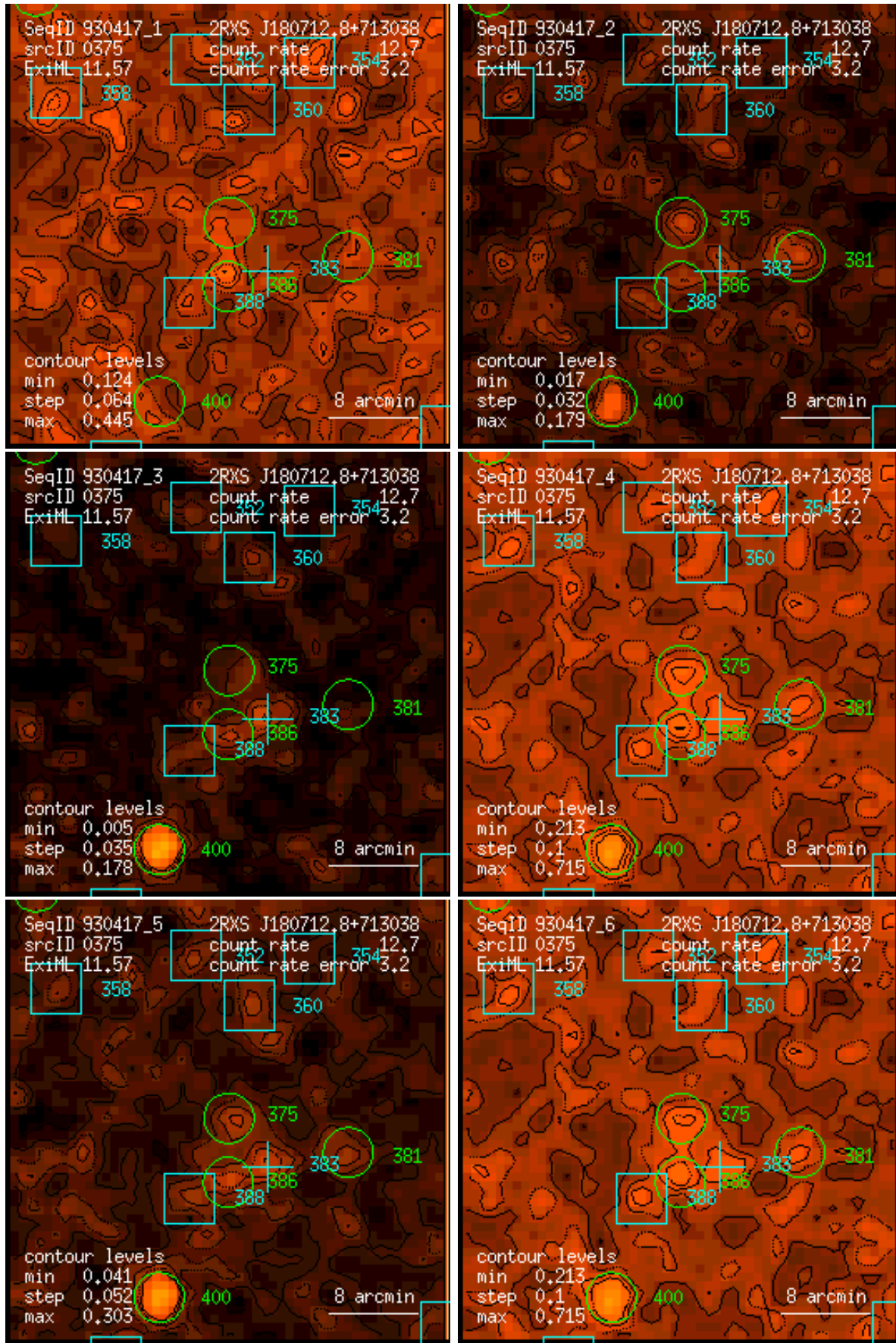
Figure 375: RASS 930417: detection 0375: band rate images, Gaussian filter: (1) PSPC channels 11 – 41, (2) 52 – 90, (3) 91 – 201, (4) 11 – 235, (5) 52 – 201, (6) 11 – 201. Broad band rates in counts/ks. Band rate contour levels in counts/ks/arcmin 2 .
