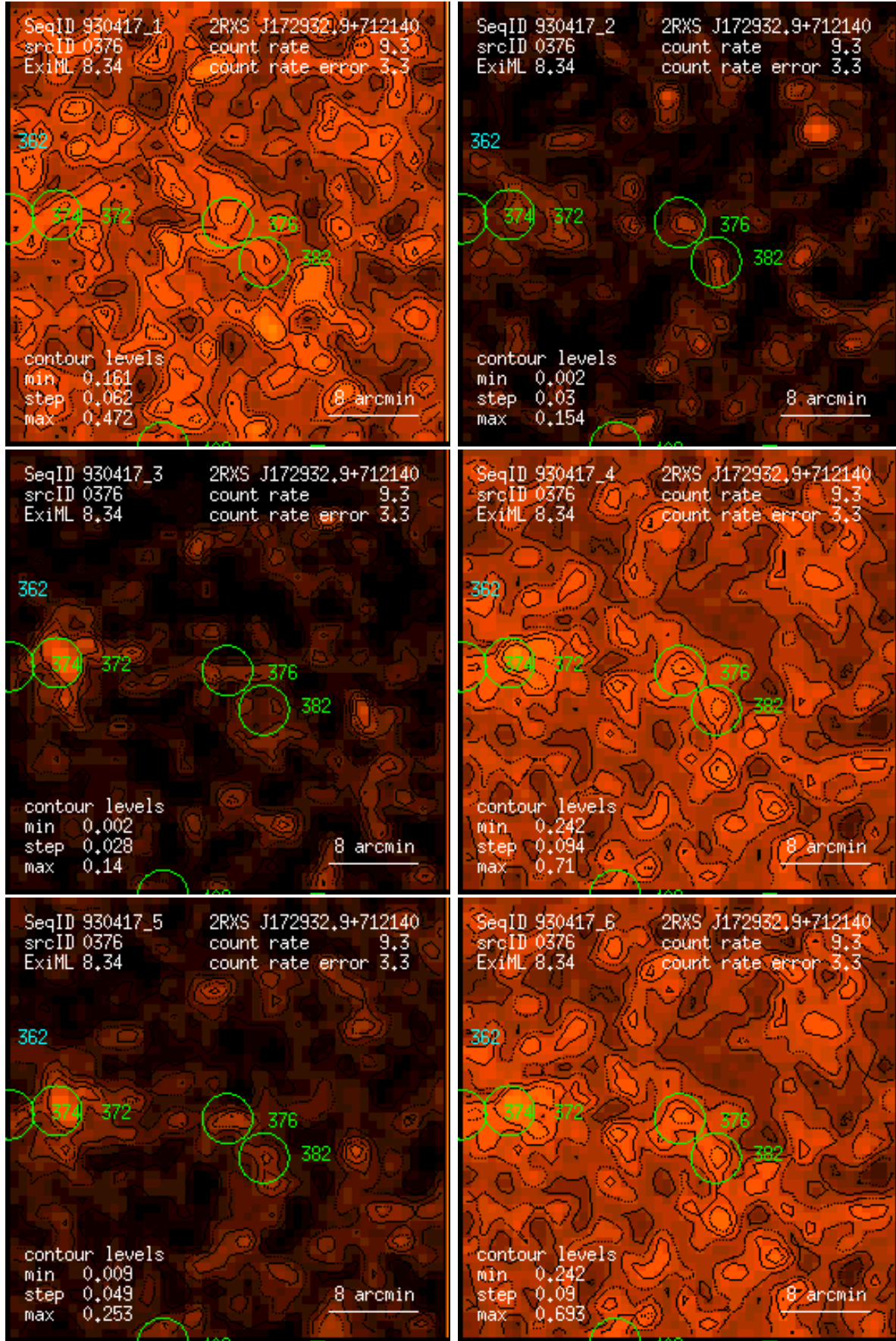
Figure 376: RASS 930417: detection 0376: band rate images, Gaussian filter: (1) PSPC channels 11 – 41, (2) 52 – 90, (3) 91 – 201, (4) 11 – 235, (5) 52 – 201, (6) 11 – 201. Broad band rates in counts/ks. Band rate contour levels in counts/ks/arcmin 2 .
