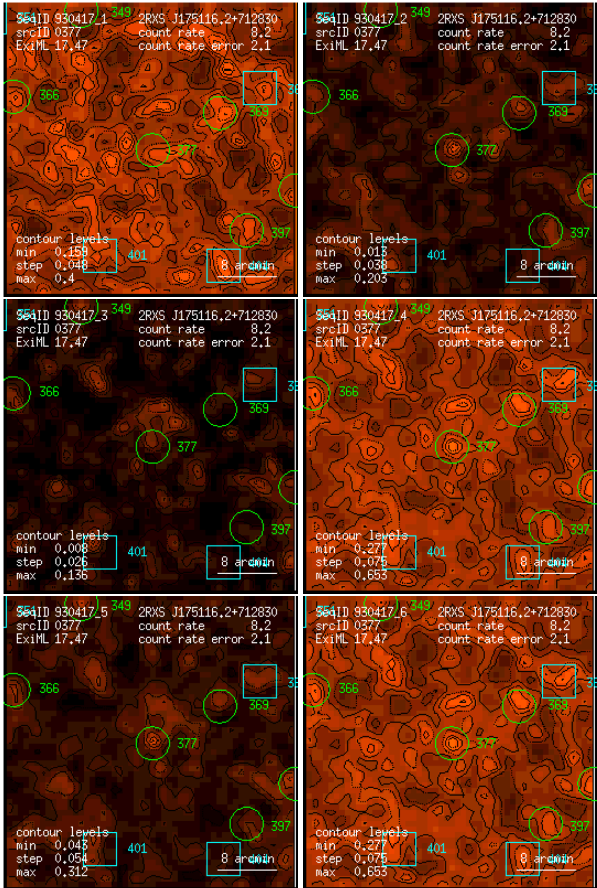
Figure 377: RASS 930417: detection 0377: band rate images, Gaussian filter: (1) PSPC channels 11 – 41, (2) 52 – 90, (3) 91 – 201, (4) 11 – 235, (5) 52 – 201, (6) 11 – 201. Broad band rates in counts/ks. Band rate contour levels in counts/ks/arcmin 2 .
