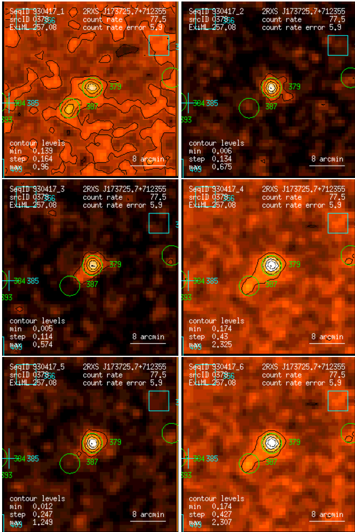
Figure 379: RASS 930417: detection 0379: band rate images, Gaussian filter: (1) PSPC channels 11 – 41, (2) 52 – 90, (3) 91 – 201, (4) 11 – 235, (5) 52 – 201, (6) 11 – 201. Broad band rates in counts/ks. Band rate contour levels in counts/ks/arcmin 2 .
