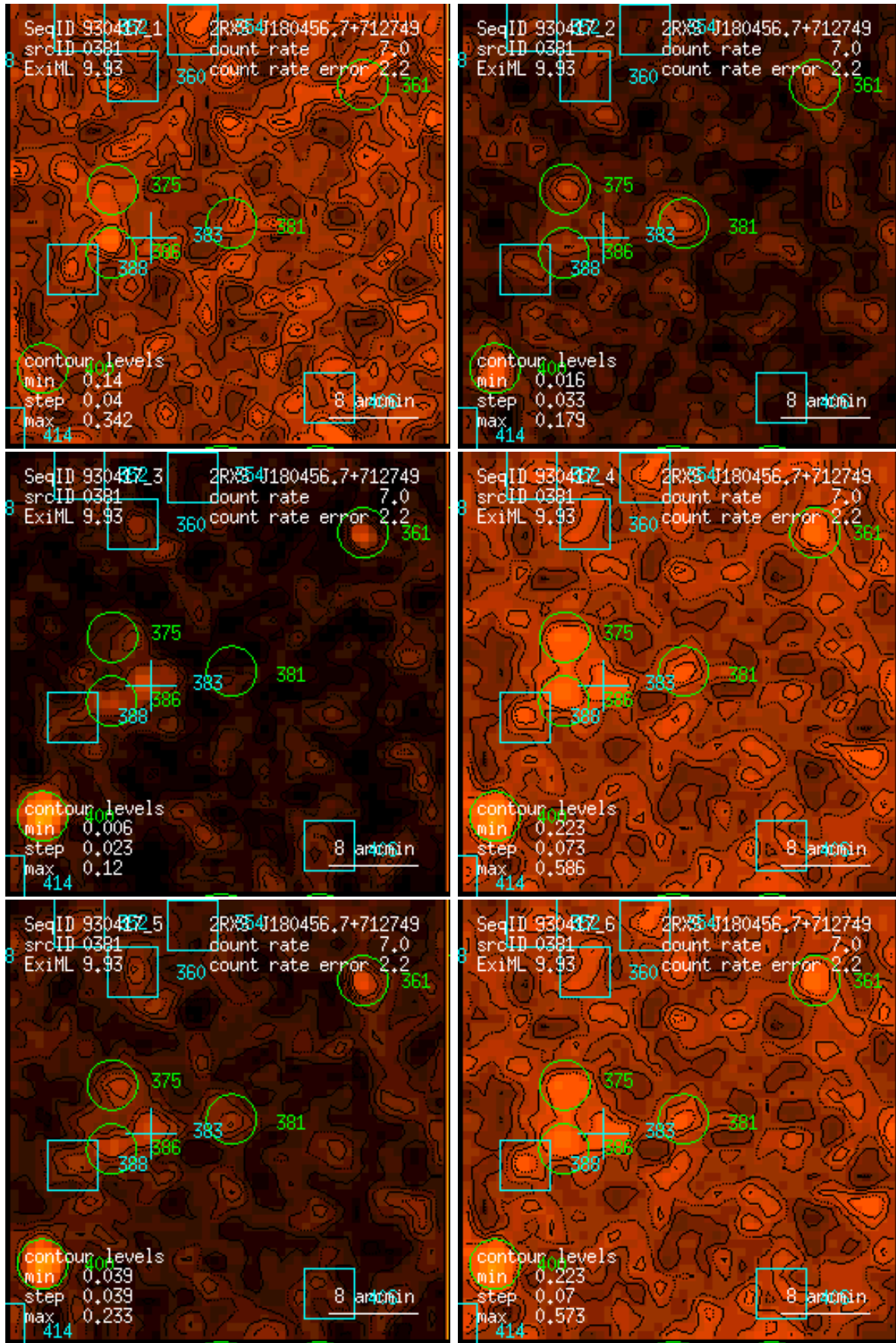
Figure 381: RASS 930417: detection 0381: band rate images, Gaussian filter: (1) PSPC channels 11 – 41, (2) 52 – 90, (3) 91 – 201, (4) 11 – 235, (5) 52 – 201, (6) 11 – 201. Broad band rates in counts/ks. Band rate contour levels in counts/ks/arcmin 2 .
