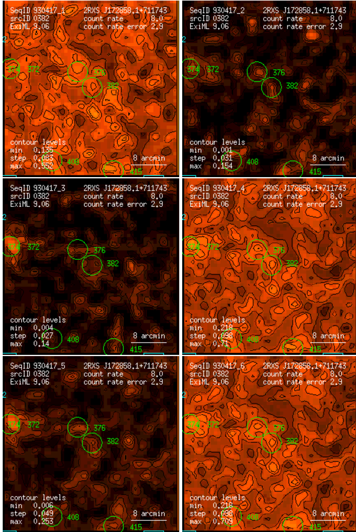
Figure 382: RASS 930417: detection 0382: band rate images, Gaussian filter: (1) PSPC channels 11 – 41, (2) 52 – 90, (3) 91 – 201, (4) 11 – 235, (5) 52 – 201, (6) 11 – 201. Broad band rates in counts/ks. Band rate contour levels in counts/ks/arcmin 2 .
