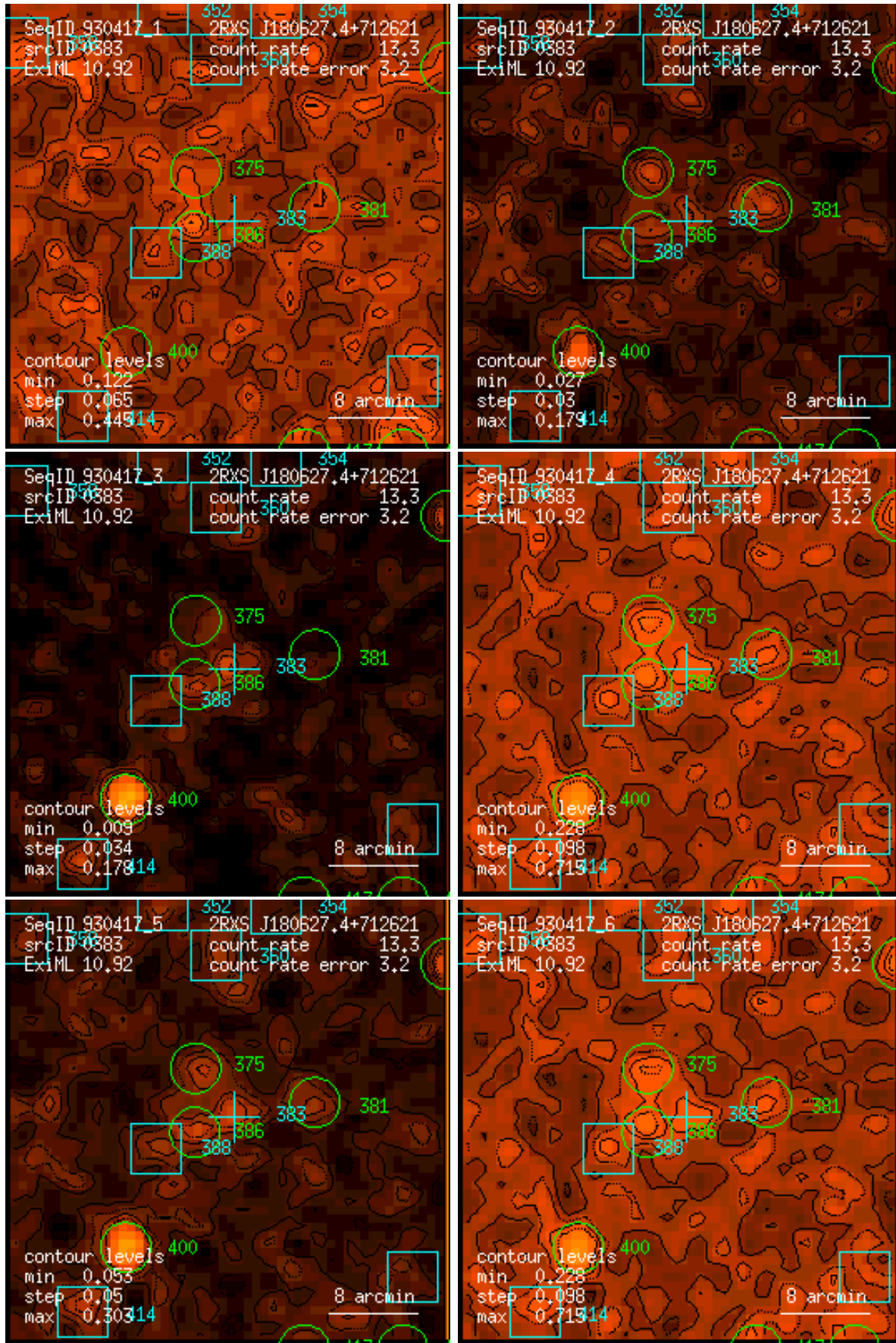
Figure 383: RASS 930417: detection 0383: band rate images, Gaussian filter: (1) PSPC channels 11 – 41, (2) 52 – 90, (3) 91 – 201, (4) 11 – 235, (5) 52 – 201, (6) 11 – 201. Broad band rates in counts/ks. Band rate contour levels in counts/ks/arcmin 2 .
