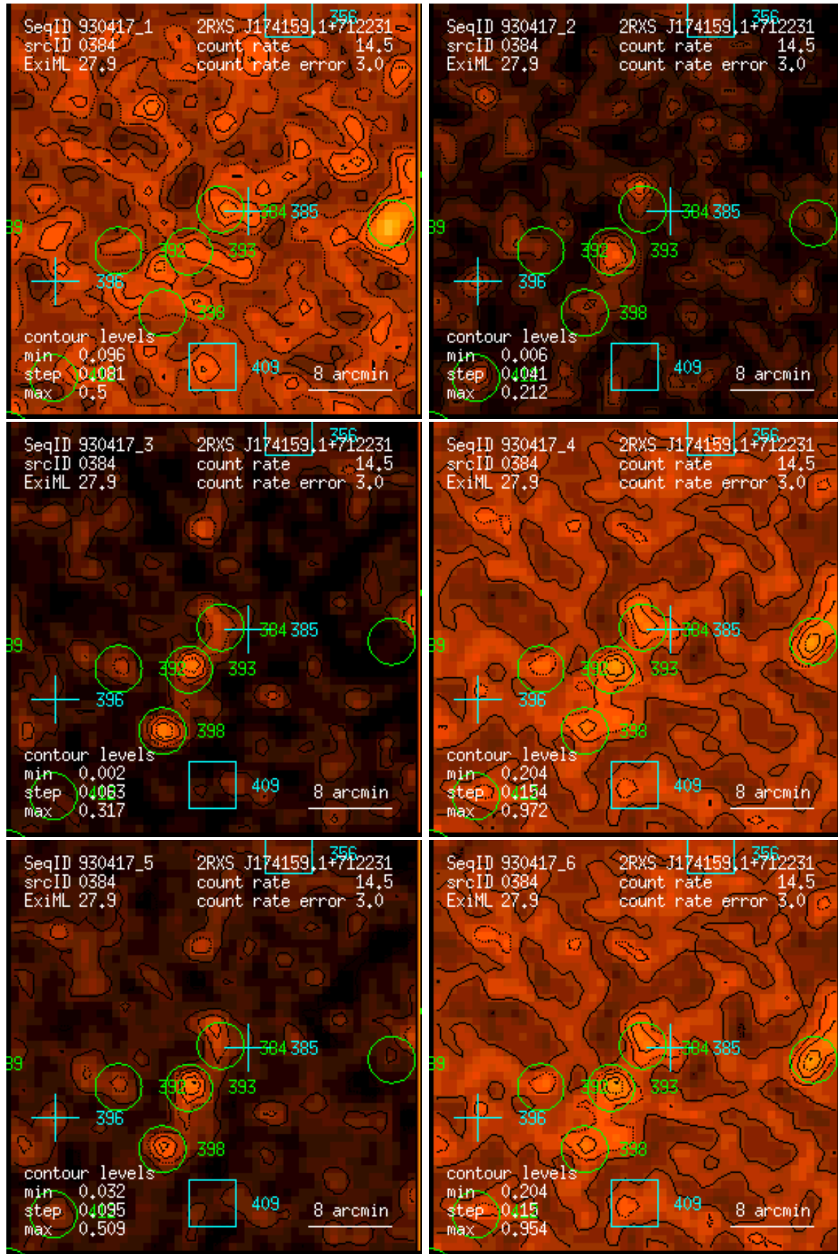
Figure 384: RASS 930417: detection 0384: band rate images, Gaussian filter: (1) PSPC channels 11 – 41, (2) 52 – 90, (3) 91 – 201, (4) 11 – 235, (5) 52 – 201, (6) 11 – 201. Broad band rates in counts/ks. Band rate contour levels in counts/ks/arcmin 2 .
