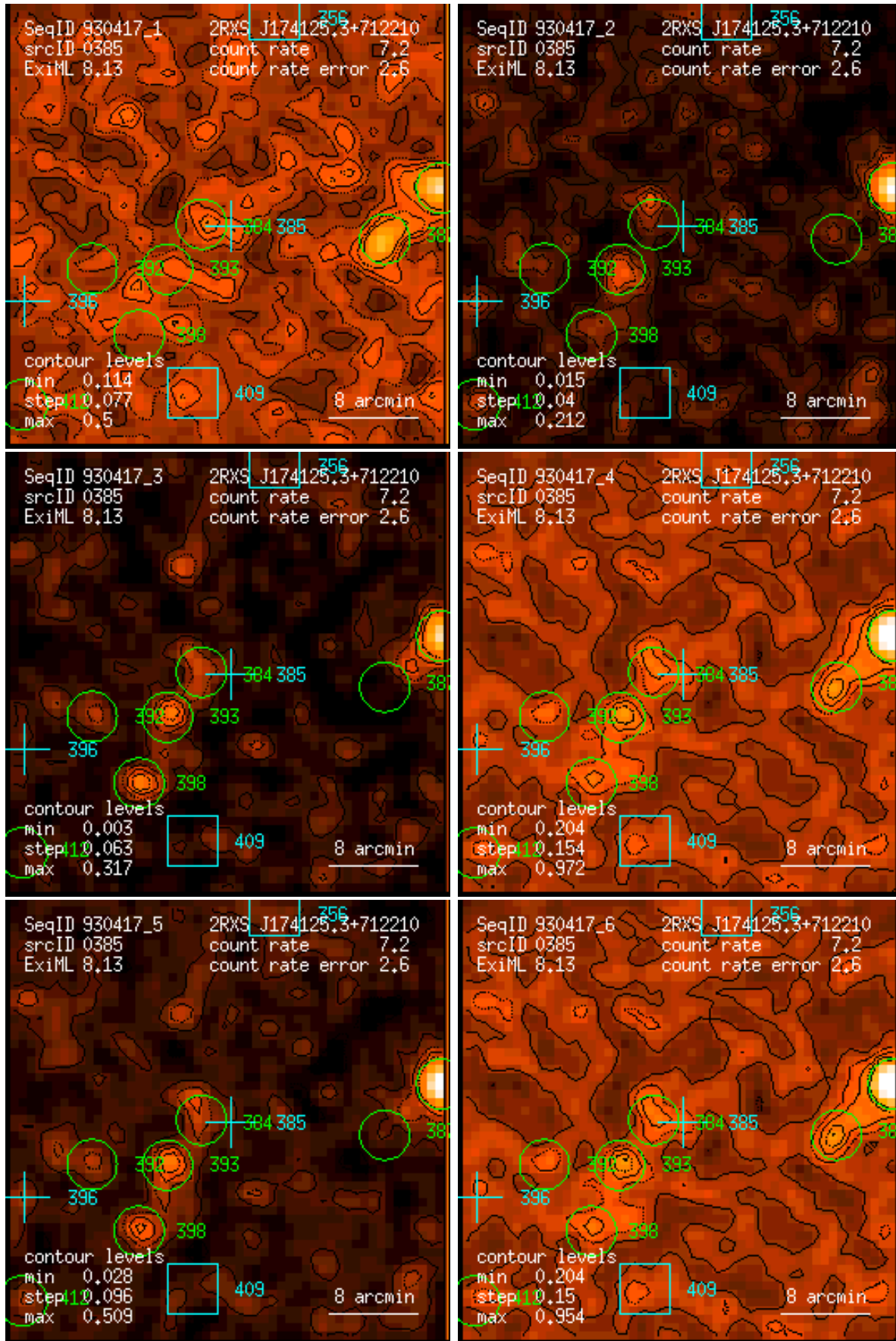
Figure 385: RASS 930417: detection 0385: band rate images, Gaussian filter: (1) PSPC channels 11 – 41, (2) 52 – 90, (3) 91 – 201, (4) 11 – 235, (5) 52 – 201, (6) 11 – 201. Broad band rates in counts/ks. Band rate contour levels in counts/ks/arcmin 2 .
