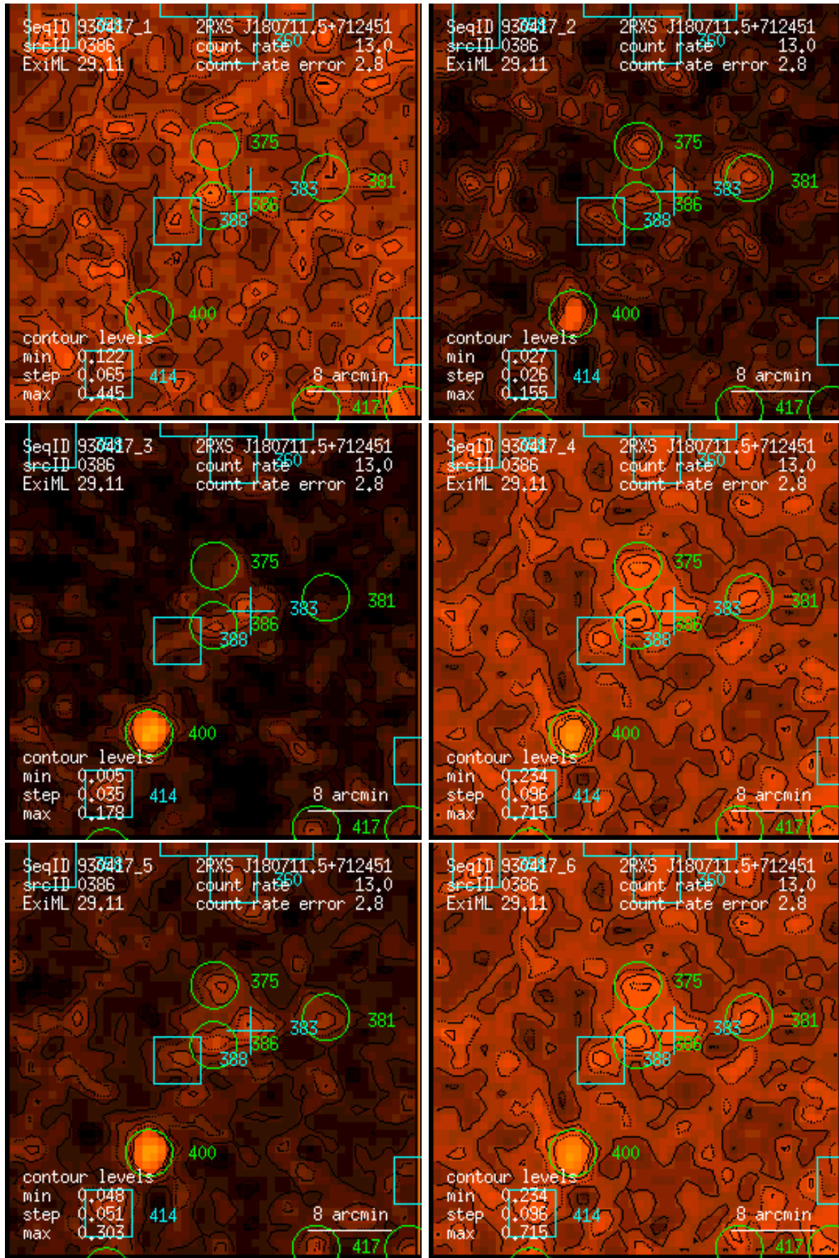
Figure 386: RASS 930417: detection 0386: band rate images, Gaussian filter: (1) PSPC channels 11 – 41, (2) 52 – 90, (3) 91 – 201, (4) 11 – 235, (5) 52 – 201, (6) 11 – 201. Broad band rates in counts/ks. Band rate contour levels in counts/ks/arcmin 2 .
