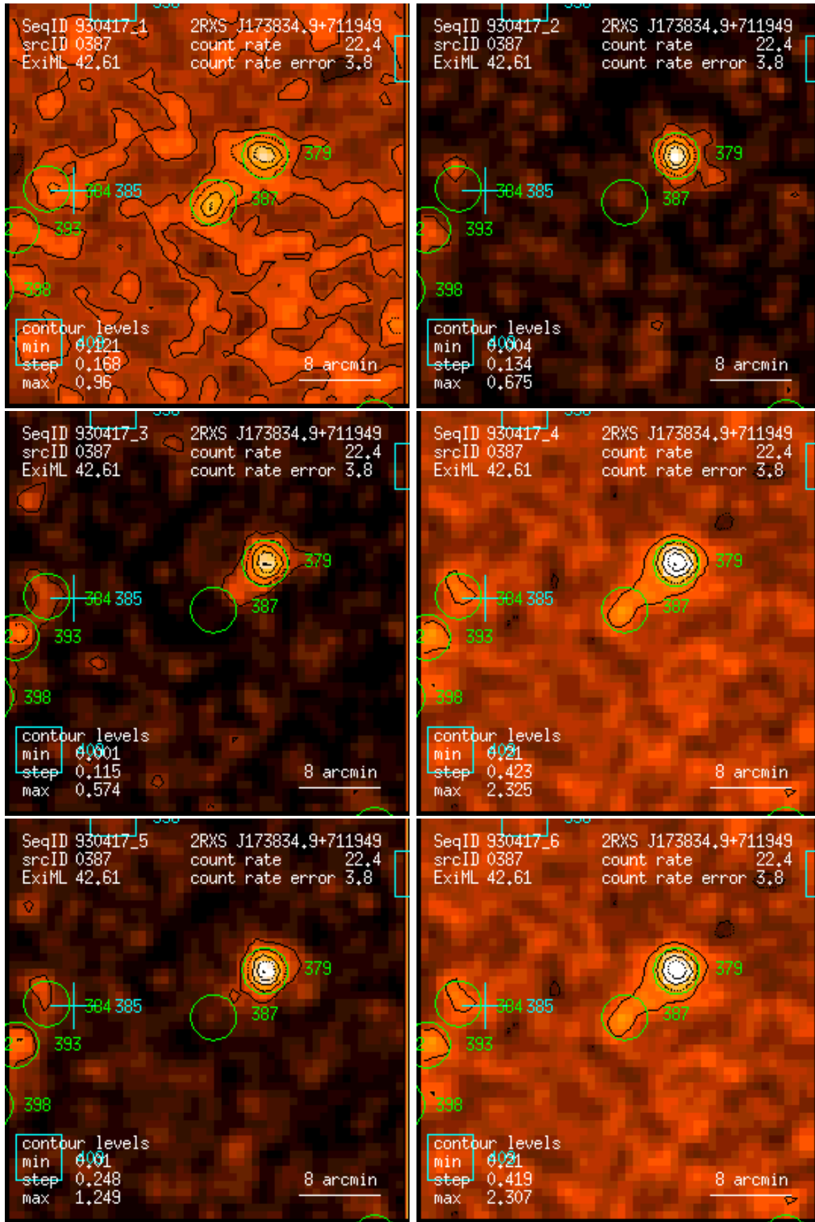
Figure 387: RASS 930417: detection 0387: band rate images, Gaussian filter: (1) PSPC channels 11 – 41, (2) 52 – 90, (3) 91 – 201, (4) 11 – 235, (5) 52 – 201, (6) 11 – 201. Broad band rates in counts/ks. Band rate contour levels in counts/ks/arcmin 2 .
