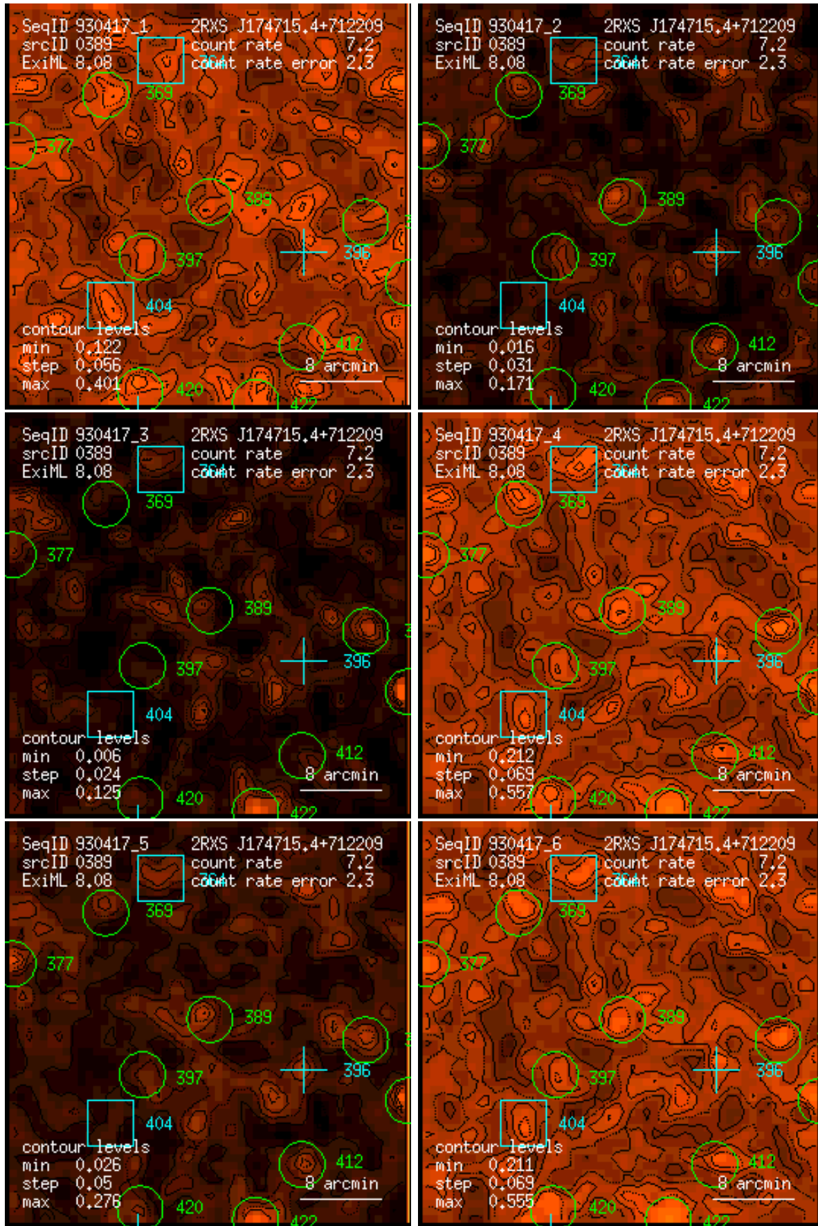
Figure 389: RASS 930417: detection 0389: band rate images, Gaussian filter: (1) PSPC channels 11 – 41, (2) 52 – 90, (3) 91 – 201, (4) 11 – 235, (5) 52 – 201, (6) 11 – 201. Broad band rates in counts/ks. Band rate contour levels in counts/ks/arcmin 2 .
