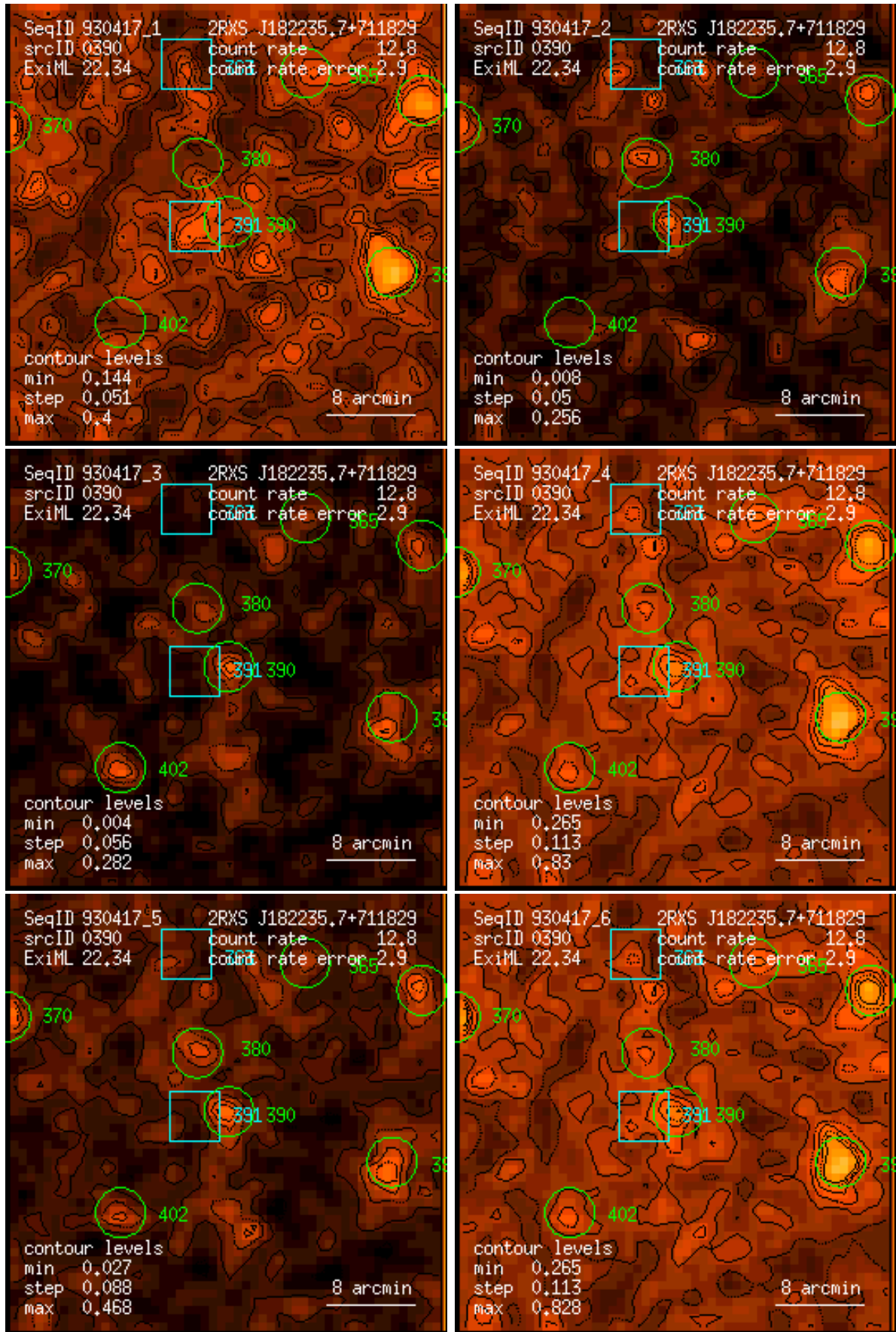
Figure 390: RASS 930417: detection 0390: band rate images, Gaussian filter: (1) PSPC channels 11 – 41, (2) 52 – 90, (3) 91 – 201, (4) 11 – 235, (5) 52 – 201, (6) 11 – 201. Broad band rates in counts/ks. Band rate contour levels in counts/ks/arcmin 2 .
