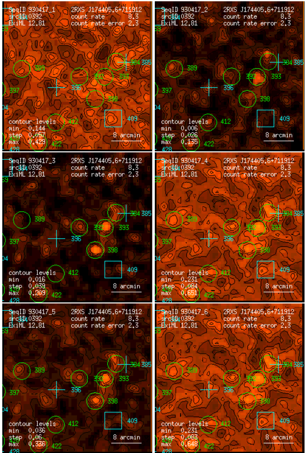
Figure 392: RASS 930417: detection 0392: band rate images, Gaussian filter: (1) PSPC channels 11 – 41, (2) 52 – 90, (3) 91 – 201, (4) 11 – 235, (5) 52 – 201, (6) 11 – 201. Broad band rates in counts/ks. Band rate contour levels in counts/ks/arcmin 2 .
