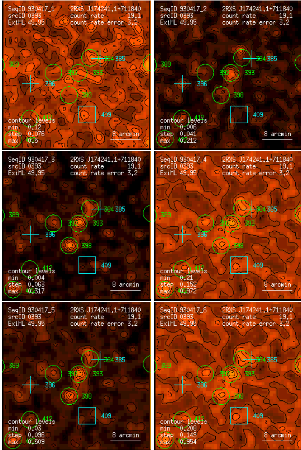
Figure 393: RASS 930417: detection 0393: band rate images, Gaussian filter: (1) PSPC channels 11 – 41, (2) 52 – 90, (3) 91 – 201, (4) 11 – 235, (5) 52 – 201, (6) 11 – 201. Broad band rates in counts/ks. Band rate contour levels in counts/ks/arcmin 2 .
