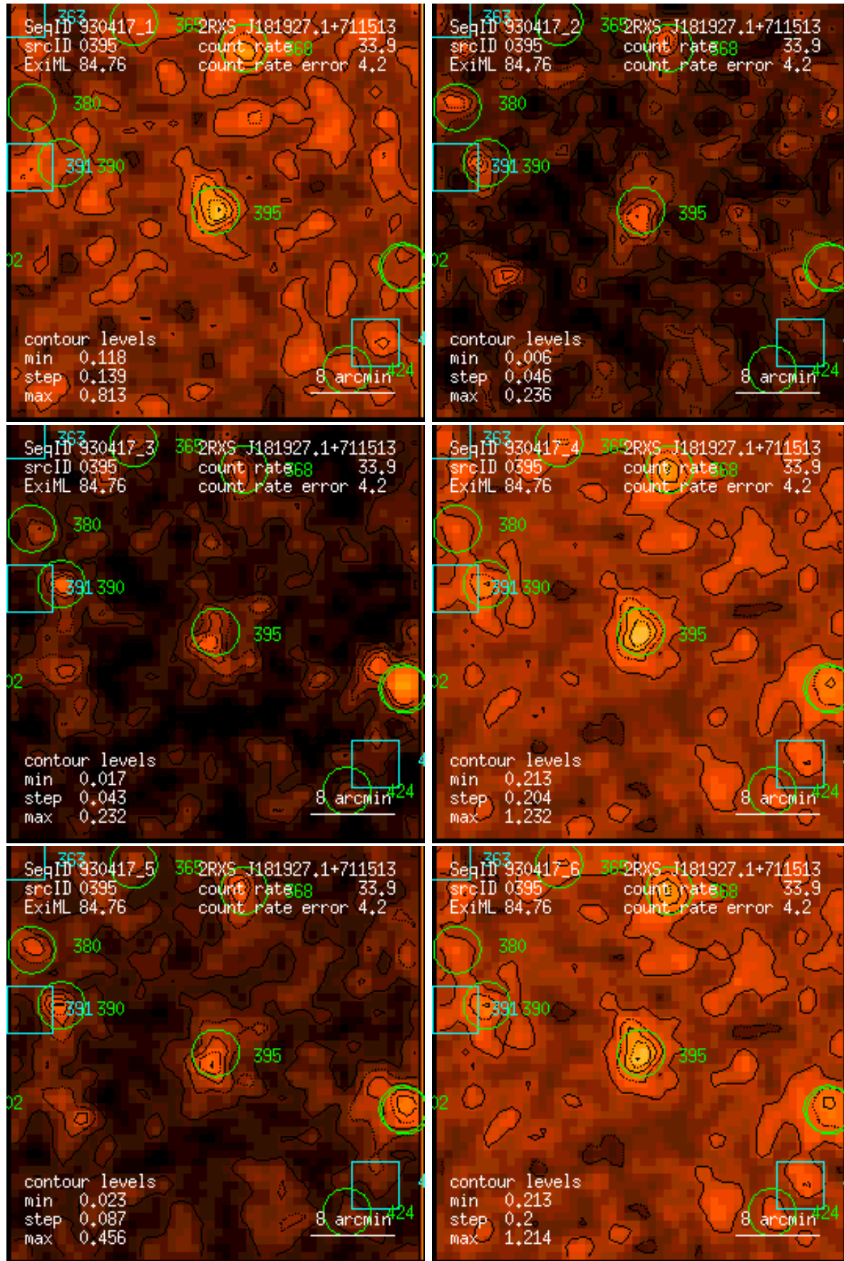
Figure 395: RASS 930417: detection 0395: band rate images, Gaussian filter: (1) PSPC channels 11 – 41, (2) 52 – 90, (3) 91 – 201, (4) 11 – 235, (5) 52 – 201, (6) 11 – 201. Broad band rates in counts/ks. Band rate contour levels in counts/ks/arcmin 2 .
