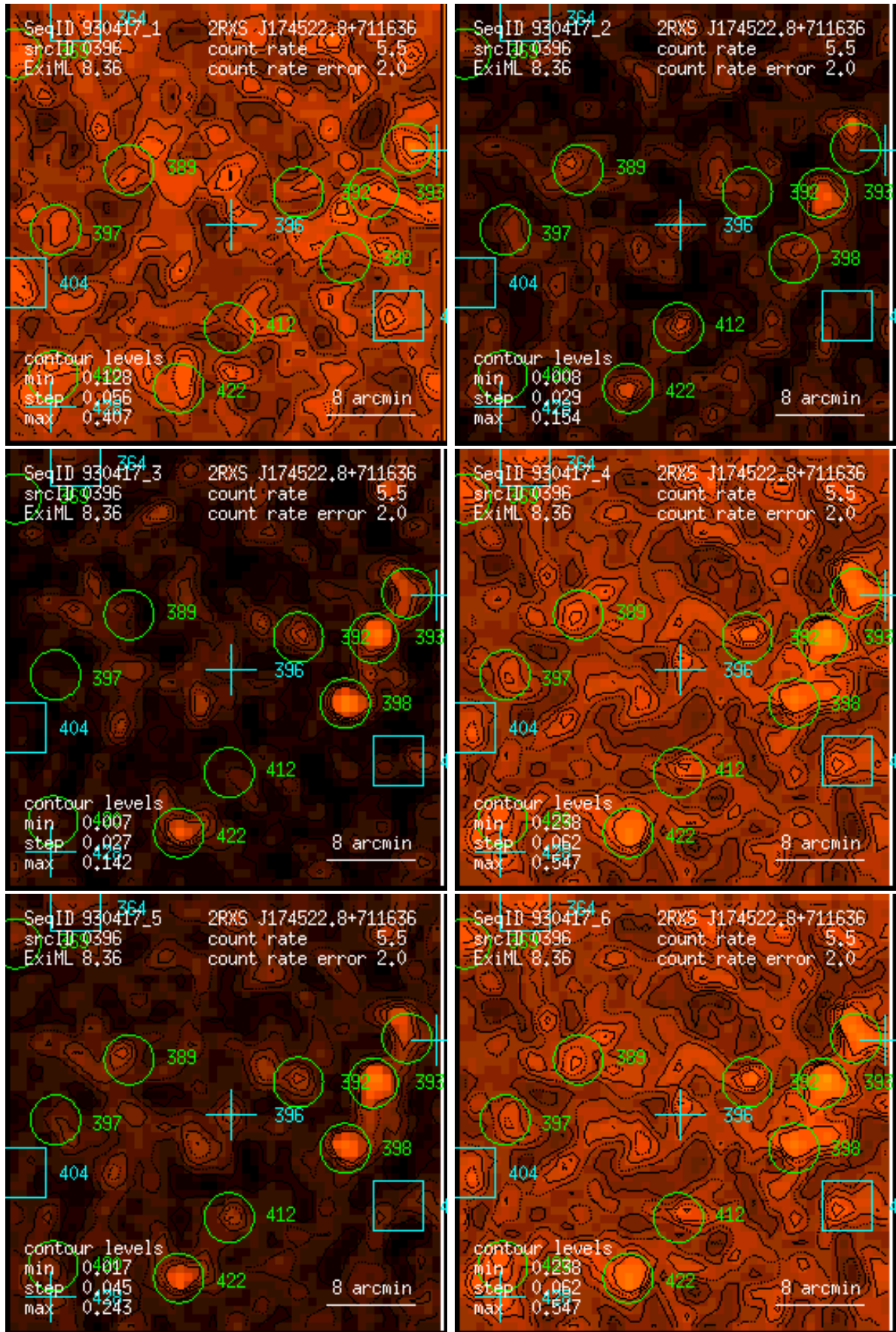
Figure 396: RASS 930417: detection 0396: band rate images, Gaussian filter: (1) PSPC channels 11 – 41, (2) 52 – 90, (3) 91 – 201, (4) 11 – 235, (5) 52 – 201, (6) 11 – 201. Broad band rates in counts/ks. Band rate contour levels in counts/ks/arcmin 2 .
