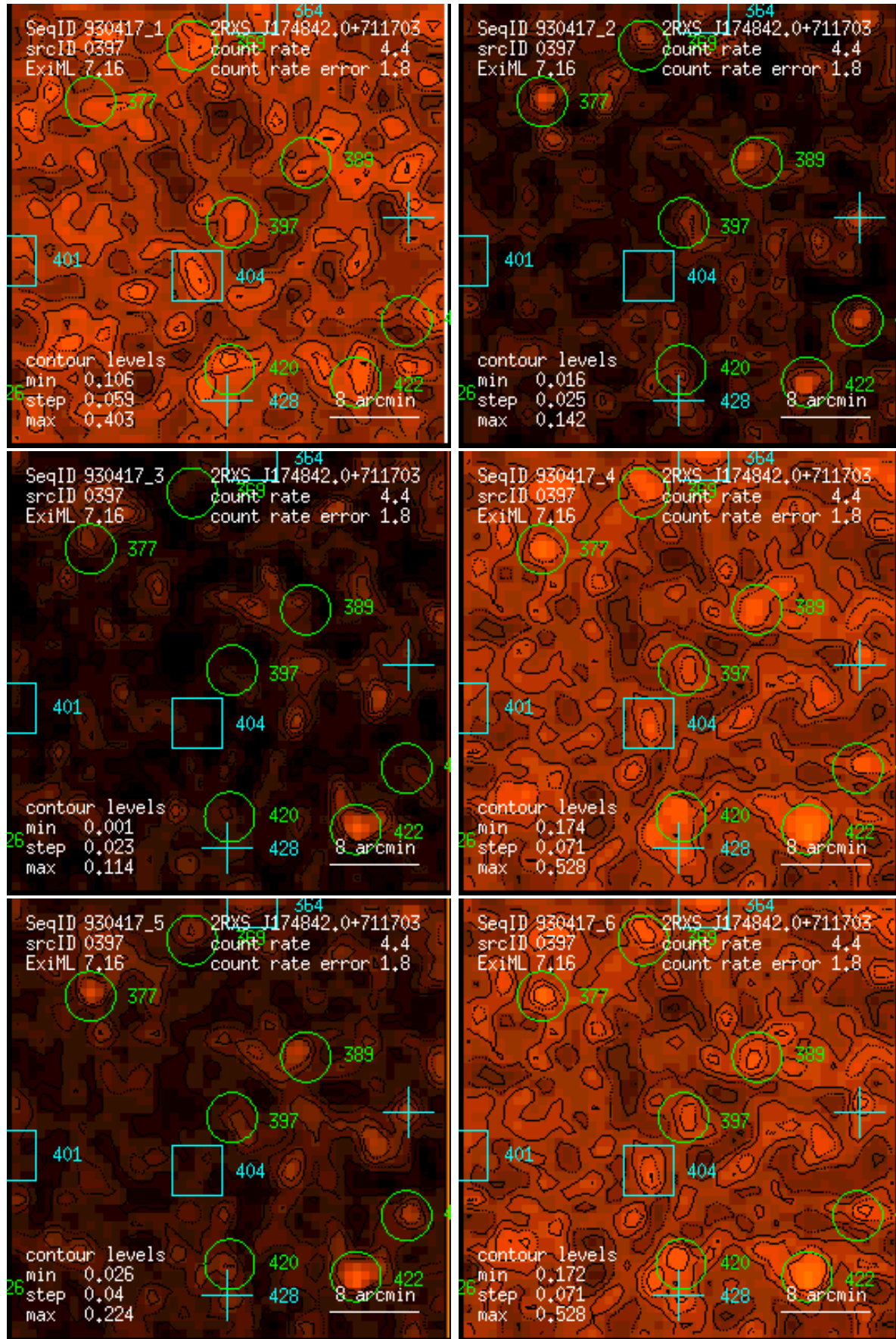
Figure 397: RASS 930417: detection 0397: band rate images, Gaussian filter: (1) PSPC channels 11 – 41, (2) 52 – 90, (3) 91 – 201, (4) 11 – 235, (5) 52 – 201, (6) 11 – 201. Broad band rates in counts/ks. Band rate contour levels in counts/ks/arcmin 2 .
