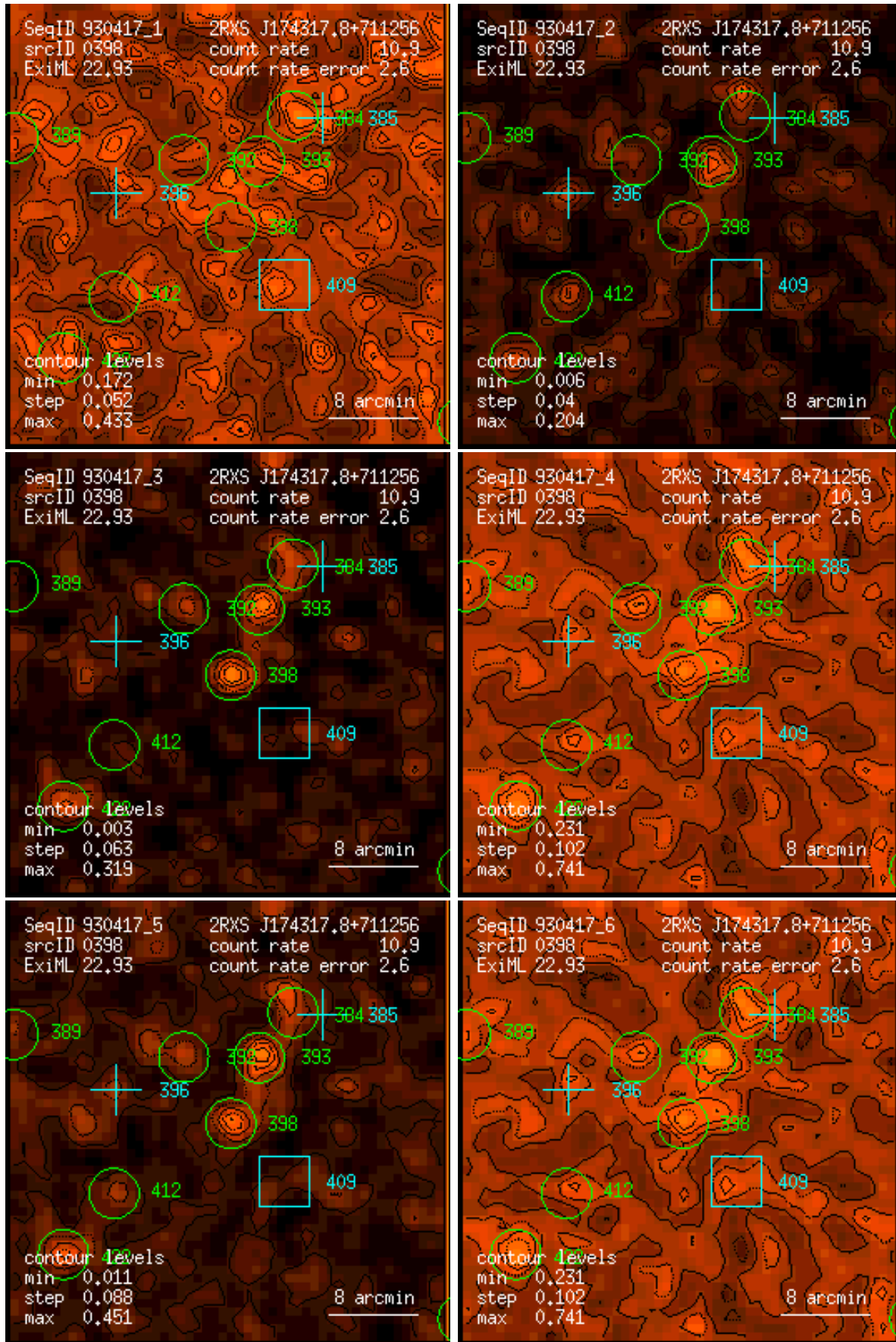
Figure 398: RASS 930417: detection 0398: band rate images, Gaussian filter: (1) PSPC channels 11 – 41, (2) 52 – 90, (3) 91 – 201, (4) 11 – 235, (5) 52 – 201, (6) 11 – 201. Broad band rates in counts/ks. Band rate contour levels in counts/ks/arcmin 2 .
