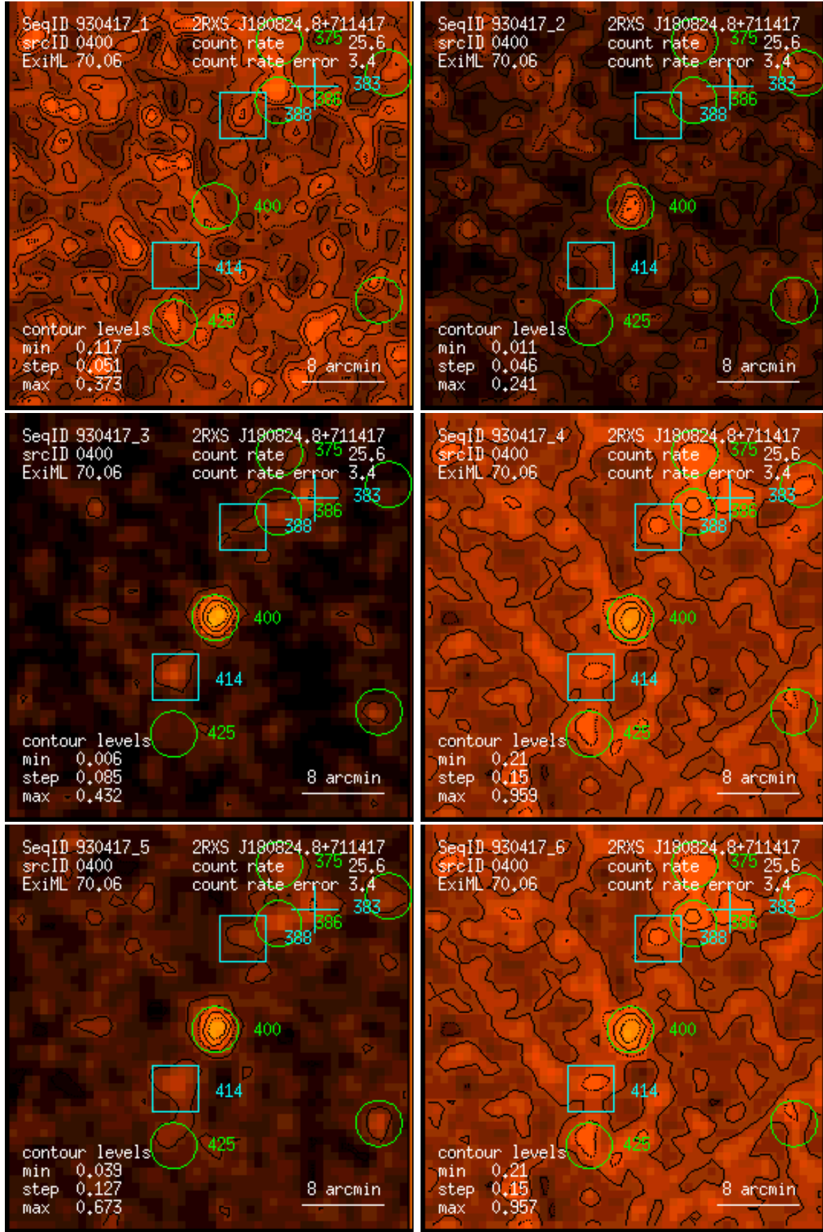
Figure 400: RASS 930417: detection 0400: band rate images, Gaussian filter: (1) PSPC channels 11 – 41, (2) 52 – 90, (3) 91 – 201, (4) 11 – 235, (5) 52 – 201, (6) 11 – 201. Broad band rates in counts/ks. Band rate contour levels in counts/ks/arcmin 2 .
