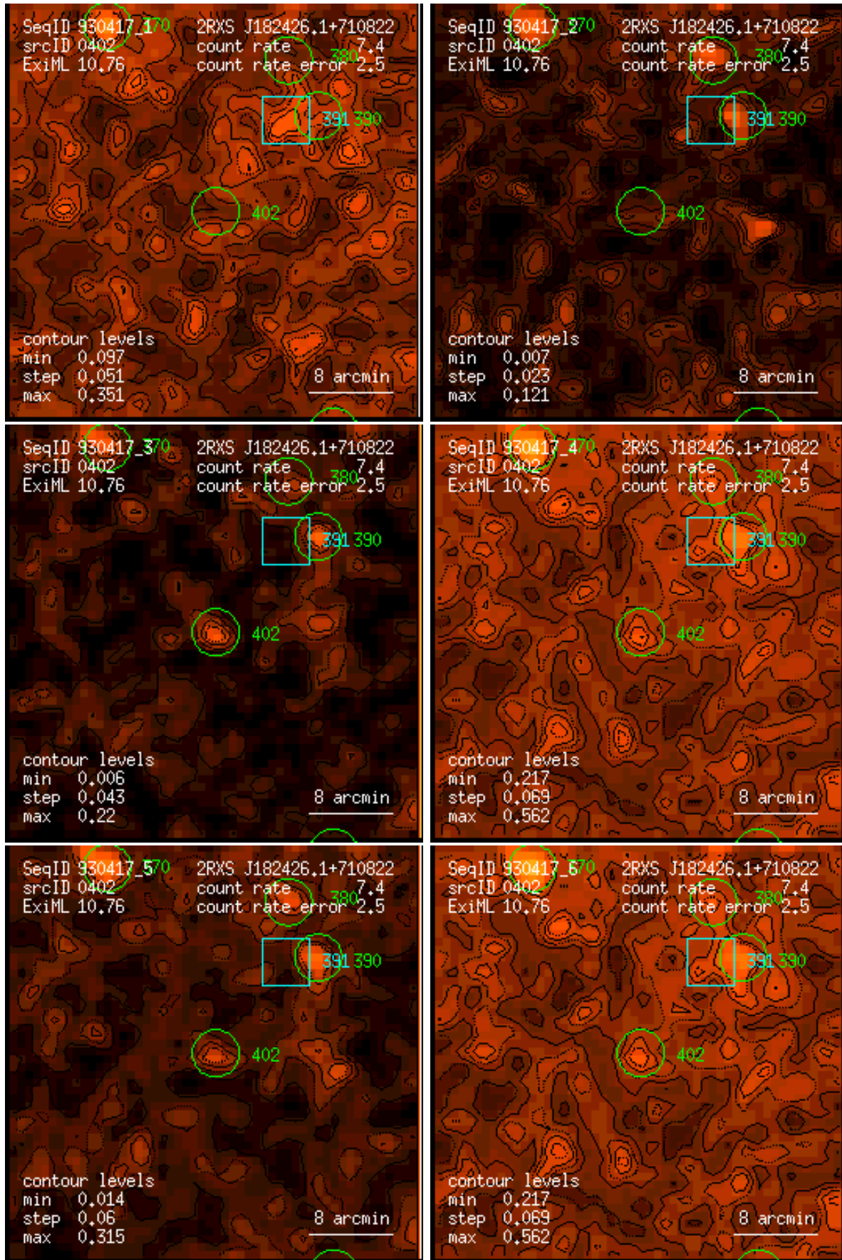
Figure 402: RASS 930417: detection 0402: band rate images, Gaussian filter: (1) PSPC channels 11 – 41, (2) 52 – 90, (3) 91 – 201, (4) 11 – 235, (5) 52 – 201, (6) 11 – 201. Broad band rates in counts/ks. Band rate contour levels in counts/ks/arcmin 2 .
