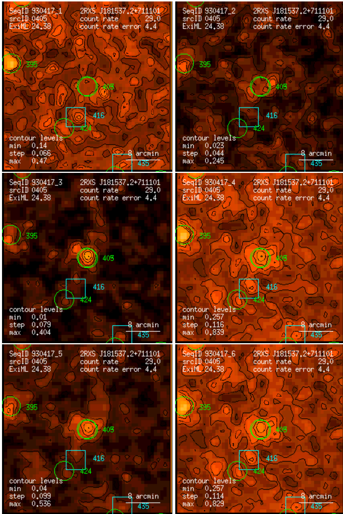
Figure 405: RASS 930417: detection 0405: band rate images, Gaussian filter: (1) PSPC channels 11 – 41, (2) 52 – 90, (3) 91 – 201, (4) 11 – 235, (5) 52 – 201, (6) 11 – 201. Broad band rates in counts/ks. Band rate contour levels in counts/ks/arcmin 2 .
