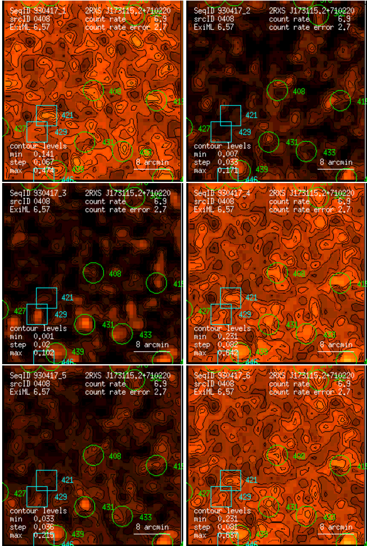
Figure 408: RASS 930417: detection 0408: band rate images, Gaussian filter: (1) PSPC channels 11 – 41, (2) 52 – 90, (3) 91 – 201, (4) 11 – 235, (5) 52 – 201, (6) 11 – 201. Broad band rates in counts/ks. Band rate contour levels in counts/ks/arcmin 2 .
