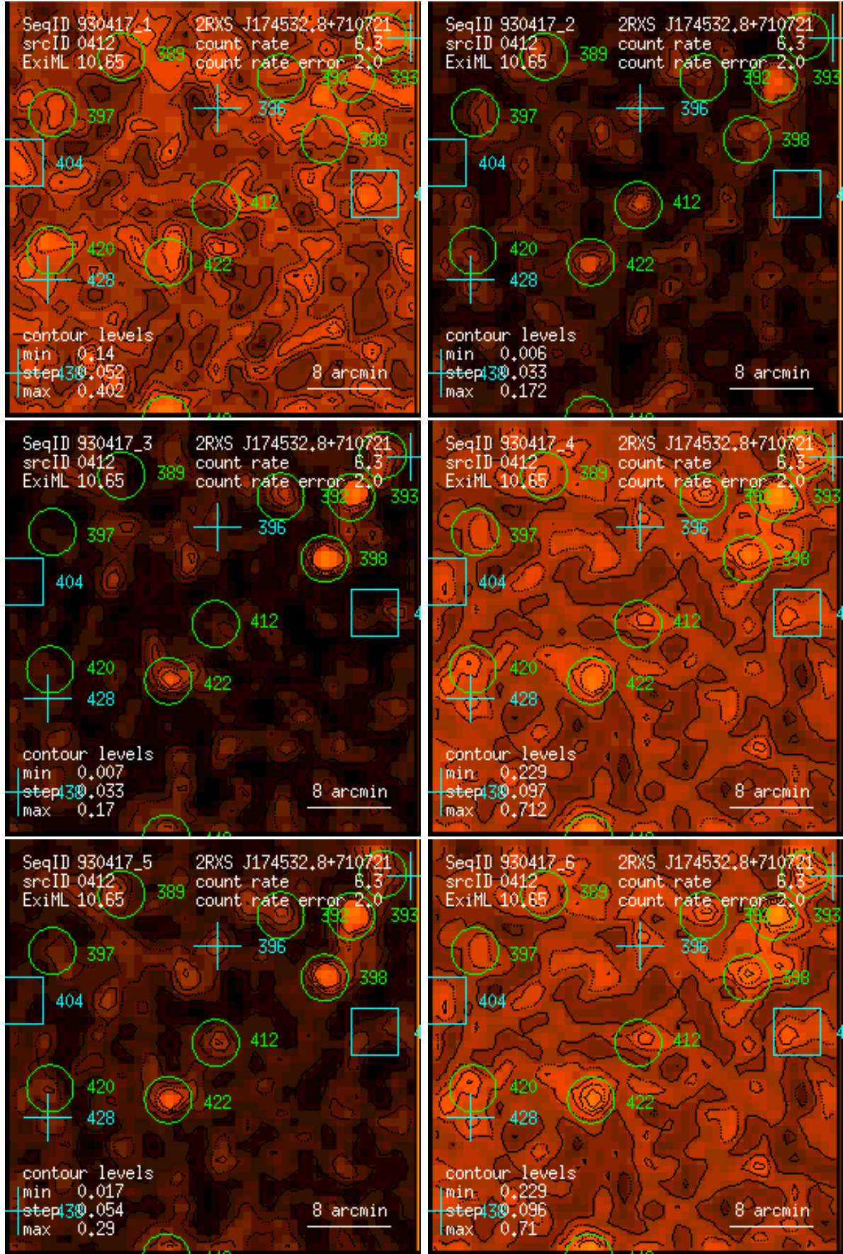
Figure 412: RASS 930417: detection 0412: band rate images, Gaussian filter: (1) PSPC channels 11 – 41, (2) 52 – 90, (3) 91 – 201, (4) 11 – 235, (5) 52 – 201, (6) 11 – 201. Broad band rates in counts/ks. Band rate contour levels in counts/ks/arcmin 2 .
