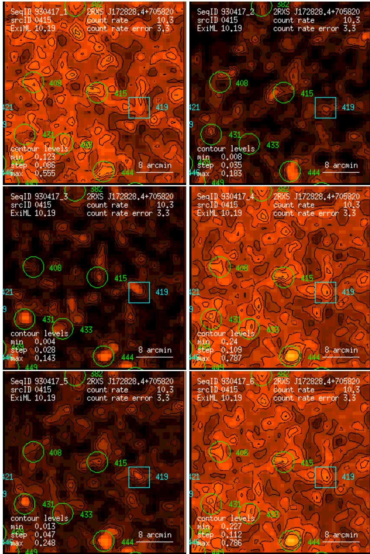
Figure 415: RASS 930417: detection 0415: band rate images, Gaussian filter: (1) PSPC channels 11 – 41, (2) 52 – 90, (3) 91 – 201, (4) 11 – 235, (5) 52 – 201, (6) 11 – 201. Broad band rates in counts/ks. Band rate contour levels in counts/ks/arcmin 2 .
