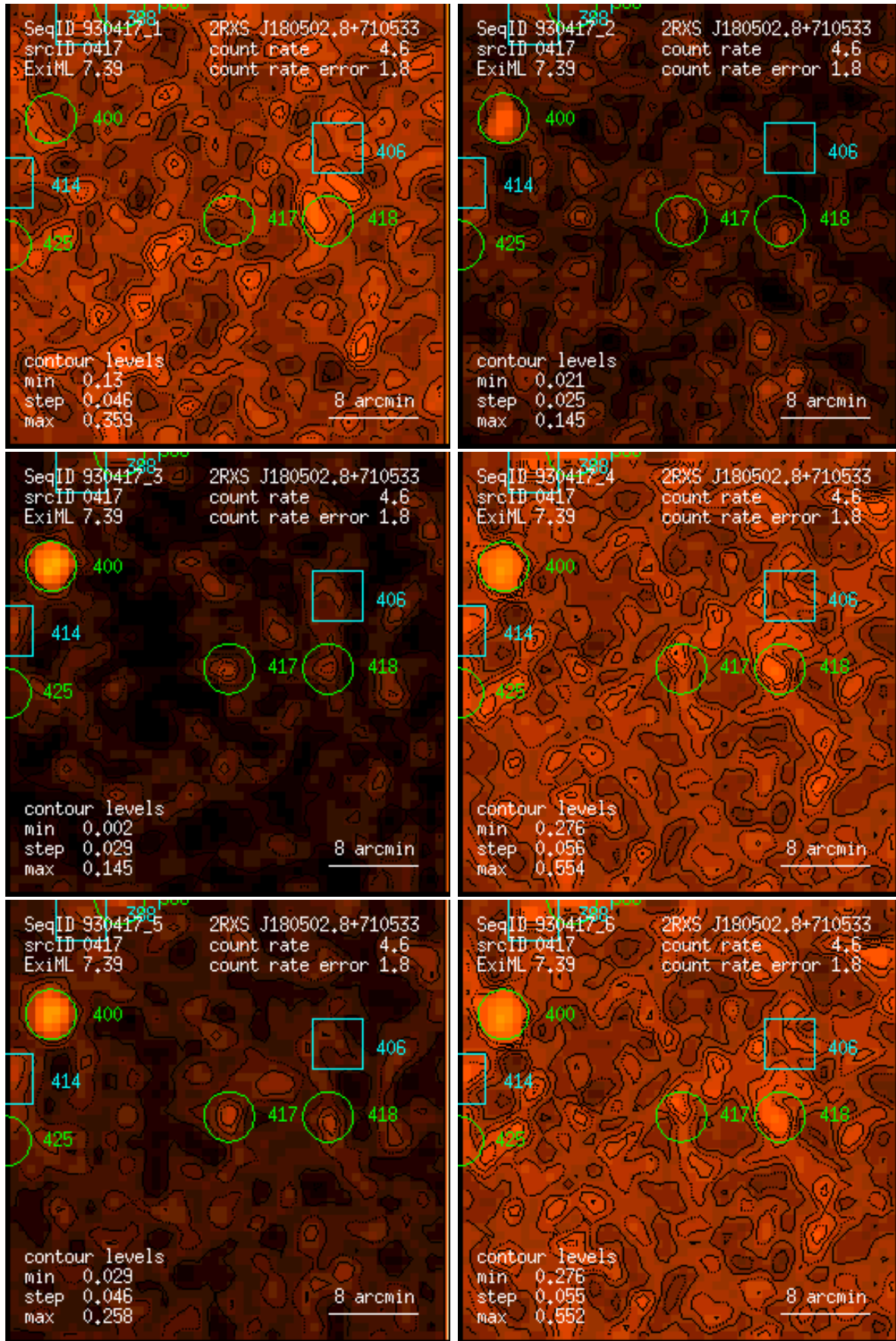
Figure 417: RASS 930417: detection 0417: band rate images, Gaussian filter: (1) PSPC channels 11 – 41, (2) 52 – 90, (3) 91 – 201, (4) 11 – 235, (5) 52 – 201, (6) 11 – 201. Broad band rates in counts/ks. Band rate contour levels in counts/ks/arcmin 2 .
