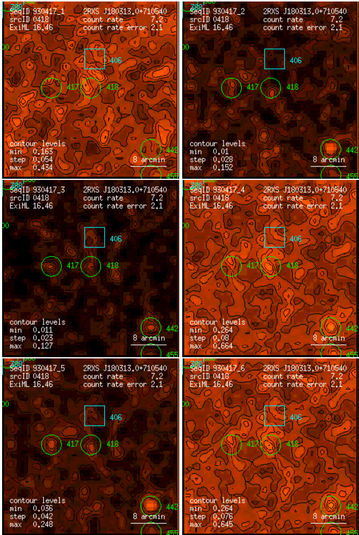
Figure 418: RASS 930417: detection 0418: band rate images, Gaussian filter: (1) PSPC channels 11 – 41, (2) 52 – 90, (3) 91 – 201, (4) 11 – 235, (5) 52 – 201, (6) 11 – 201. Broad band rates in counts/ks. Band rate contour levels in counts/ks/arcmin 2 .
