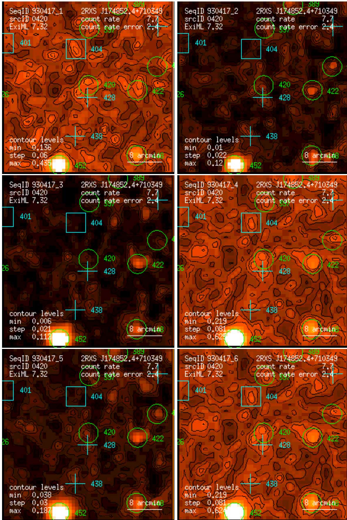
Figure 420: RASS 930417: detection 0420: band rate images, Gaussian filter: (1) PSPC channels 11 – 41, (2) 52 – 90, (3) 91 – 201, (4) 11 – 235, (5) 52 – 201, (6) 11 – 201. Broad band rates in counts/ks. Band rate contour levels in counts/ks/arcmin 2 .
