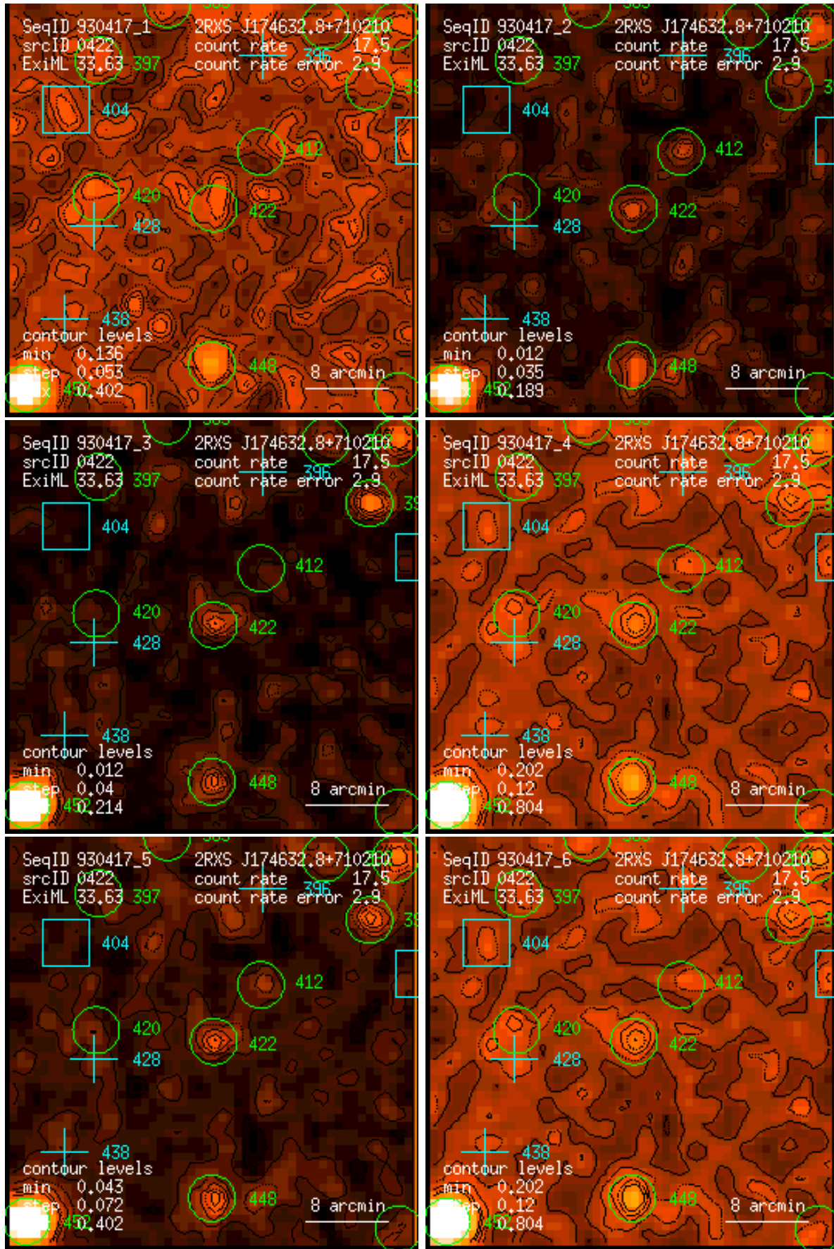
Figure 422: RASS 930417: detection 0422: band rate images, Gaussian filter: (1) PSPC channels 11 – 41, (2) 52 – 90, (3) 91 – 201, (4) 11 – 235, (5) 52 – 201, (6) 11 – 201. Broad band rates in counts/ks. Band rate contour levels in counts/ks/arcmin 2 .
