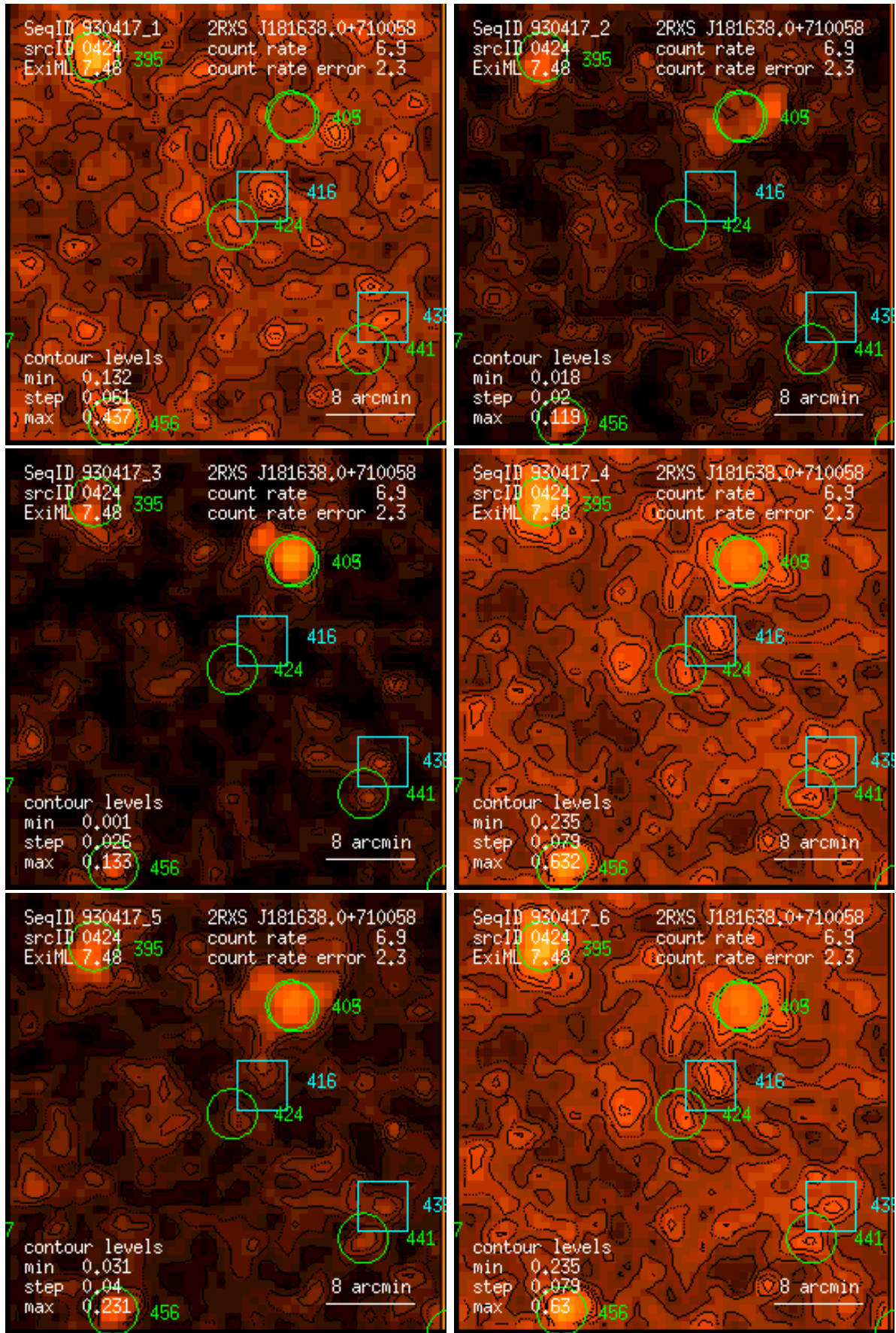
Figure 424: RASS 930417: detection 0424: band rate images, Gaussian filter: (1) PSPC channels 11 – 41, (2) 52 – 90, (3) 91 – 201, (4) 11 – 235, (5) 52 – 201, (6) 11 – 201. Broad band rates in counts/ks. Band rate contour levels in counts/ks/arcmin 2 .
