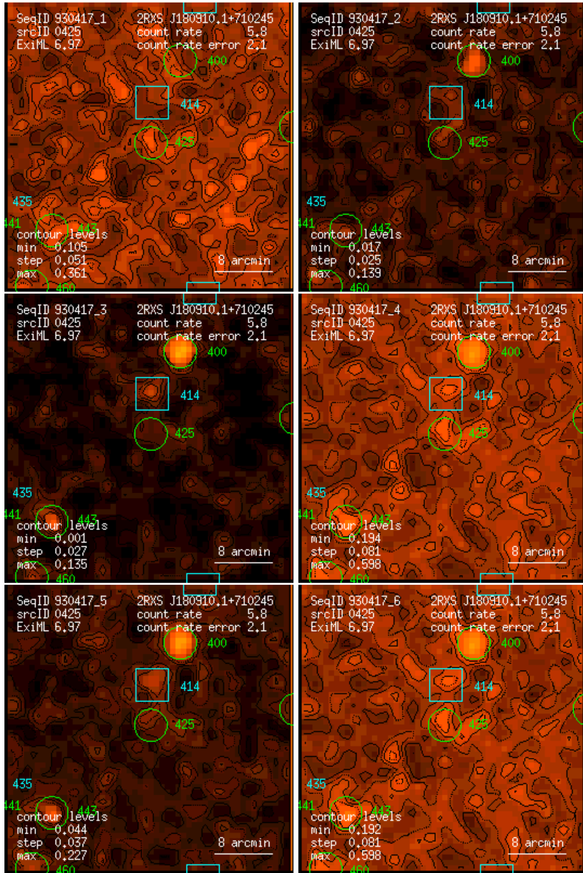
Figure 425: RASS 930417: detection 0425: band rate images, Gaussian filter: (1) PSPC channels 11 – 41, (2) 52 – 90, (3) 91 – 201, (4) 11 – 235, (5) 52 – 201, (6) 11 – 201. Broad band rates in counts/ks. Band rate contour levels in counts/ks/arcmin 2 .
