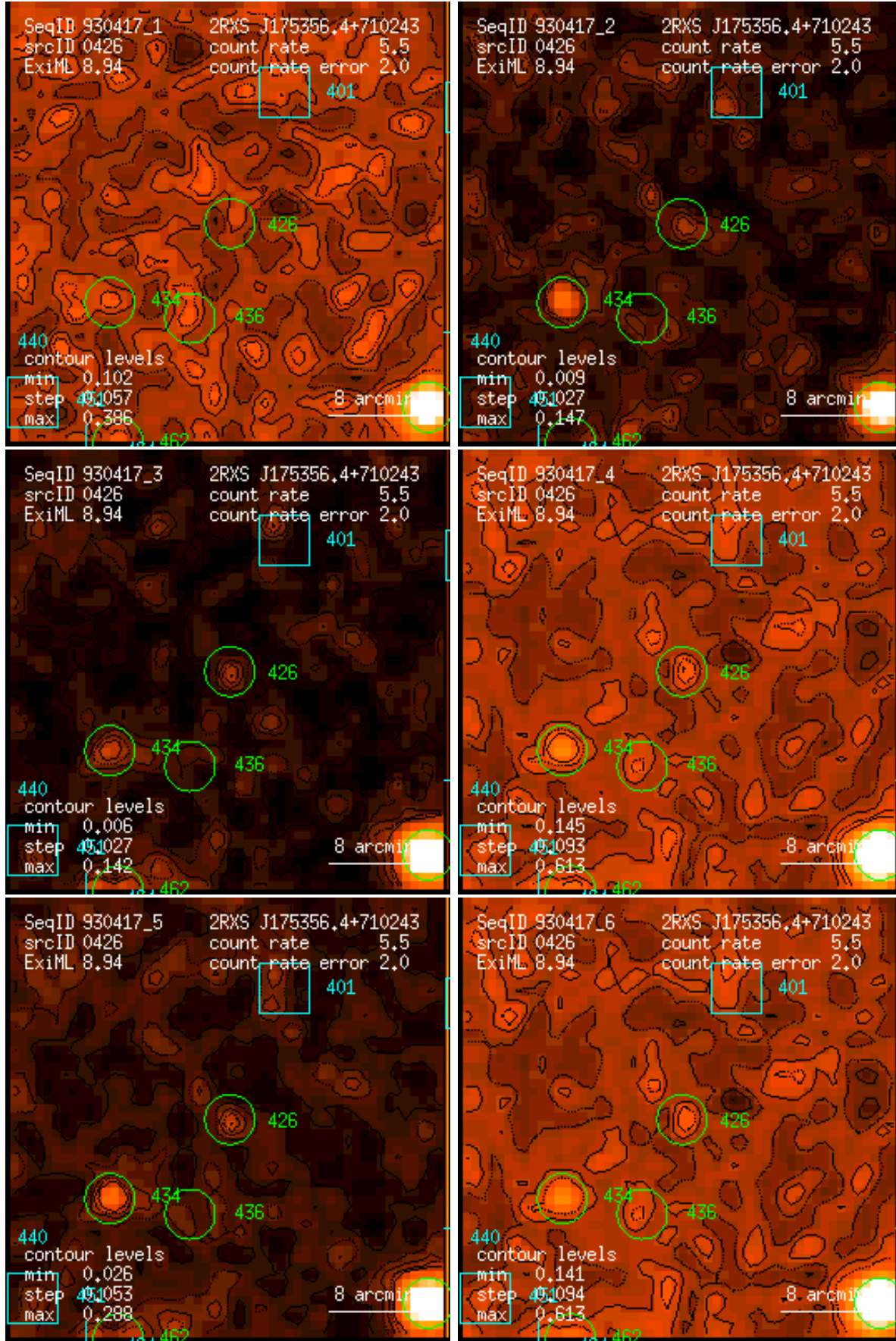
Figure 426: RASS 930417: detection 0426: band rate images, Gaussian filter: (1) PSPC channels 11 – 41, (2) 52 – 90, (3) 91 – 201, (4) 11 – 235, (5) 52 – 201, (6) 11 – 201. Broad band rates in counts/ks. Band rate contour levels in counts/ks/arcmin 2 .
