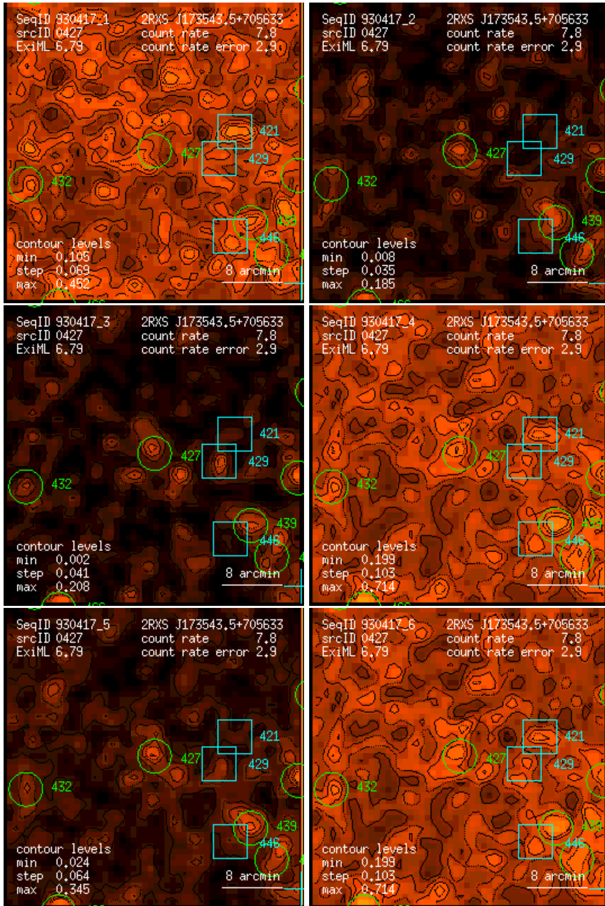
Figure 427: RASS 930417: detection 0427: band rate images, Gaussian filter: (1) PSPC channels 11 – 41, (2) 52 – 90, (3) 91 – 201, (4) 11 – 235, (5) 52 – 201, (6) 11 – 201. Broad band rates in counts/ks. Band rate contour levels in counts/ks/arcmin 2 .
