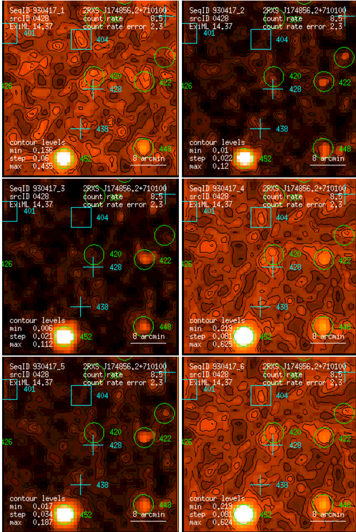
Figure 428: RASS 930417: detection 0428: band rate images, Gaussian filter: (1) PSPC channels 11 – 41, (2) 52 – 90, (3) 91 – 201, (4) 11 – 235, (5) 52 – 201, (6) 11 – 201. Broad band rates in counts/ks. Band rate contour levels in counts/ks/arcmin 2 .
