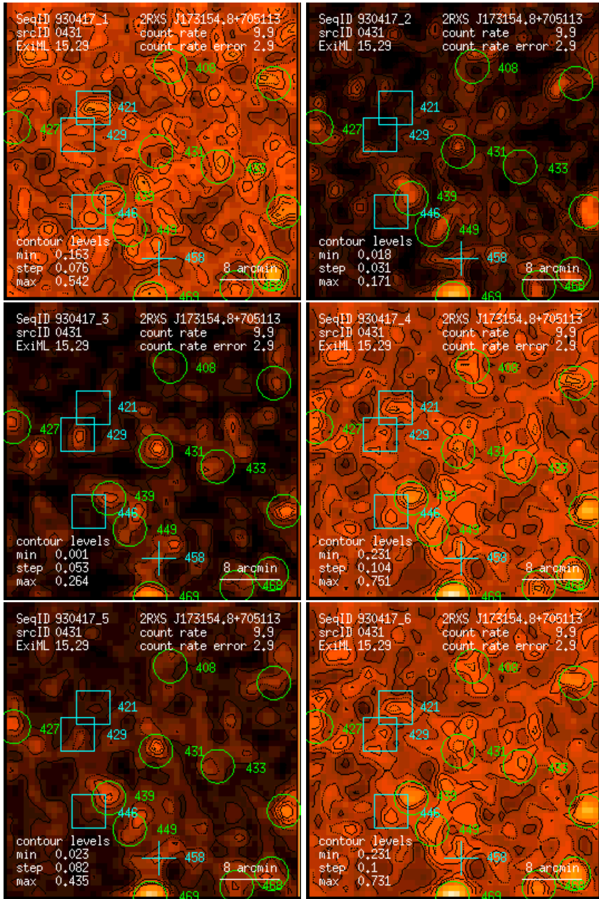
Figure 431: RASS 930417: detection 0431: band rate images, Gaussian filter: (1) PSPC channels 11 – 41, (2) 52 – 90, (3) 91 – 201, (4) 11 – 235, (5) 52 – 201, (6) 11 – 201. Broad band rates in counts/ks. Band rate contour levels in counts/ks/arcmin 2 .
