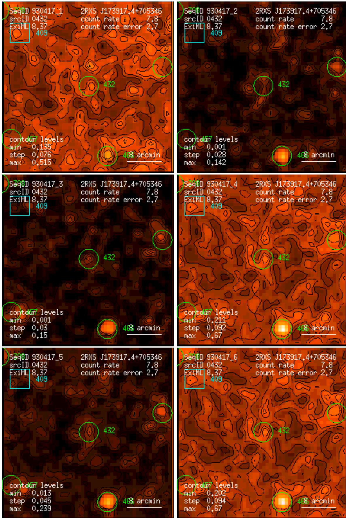
Figure 432: RASS 930417: detection 0432: band rate images, Gaussian filter: (1) PSPC channels 11 – 41, (2) 52 – 90, (3) 91 – 201, (4) 11 – 235, (5) 52 – 201, (6) 11 – 201. Broad band rates in counts/ks. Band rate contour levels in counts/ks/arcmin 2 .
