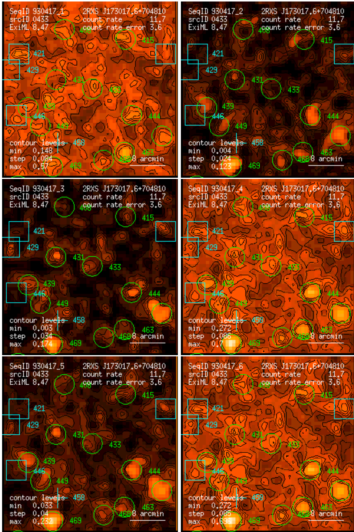
Figure 433: RASS 930417: detection 0433: band rate images, Gaussian filter: (1) PSPC channels 11 – 41, (2) 52 – 90, (3) 91 – 201, (4) 11 – 235, (5) 52 – 201, (6) 11 – 201. Broad band rates in counts/ks. Band rate contour levels in counts/ks/arcmin 2 .
