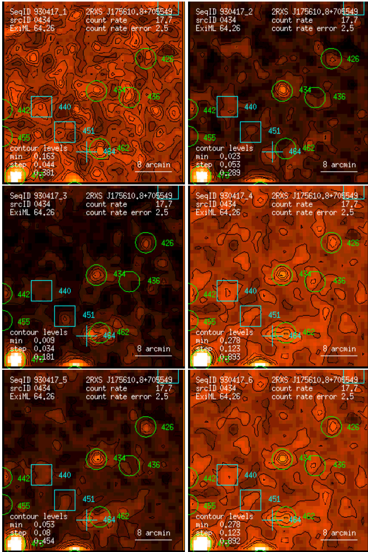
Figure 434: RASS 930417: detection 0434: band rate images, Gaussian filter: (1) PSPC channels 11 – 41, (2) 52 – 90, (3) 91 – 201, (4) 11 – 235, (5) 52 – 201, (6) 11 – 201. Broad band rates in counts/ks. Band rate contour levels in counts/ks/arcmin 2 .
