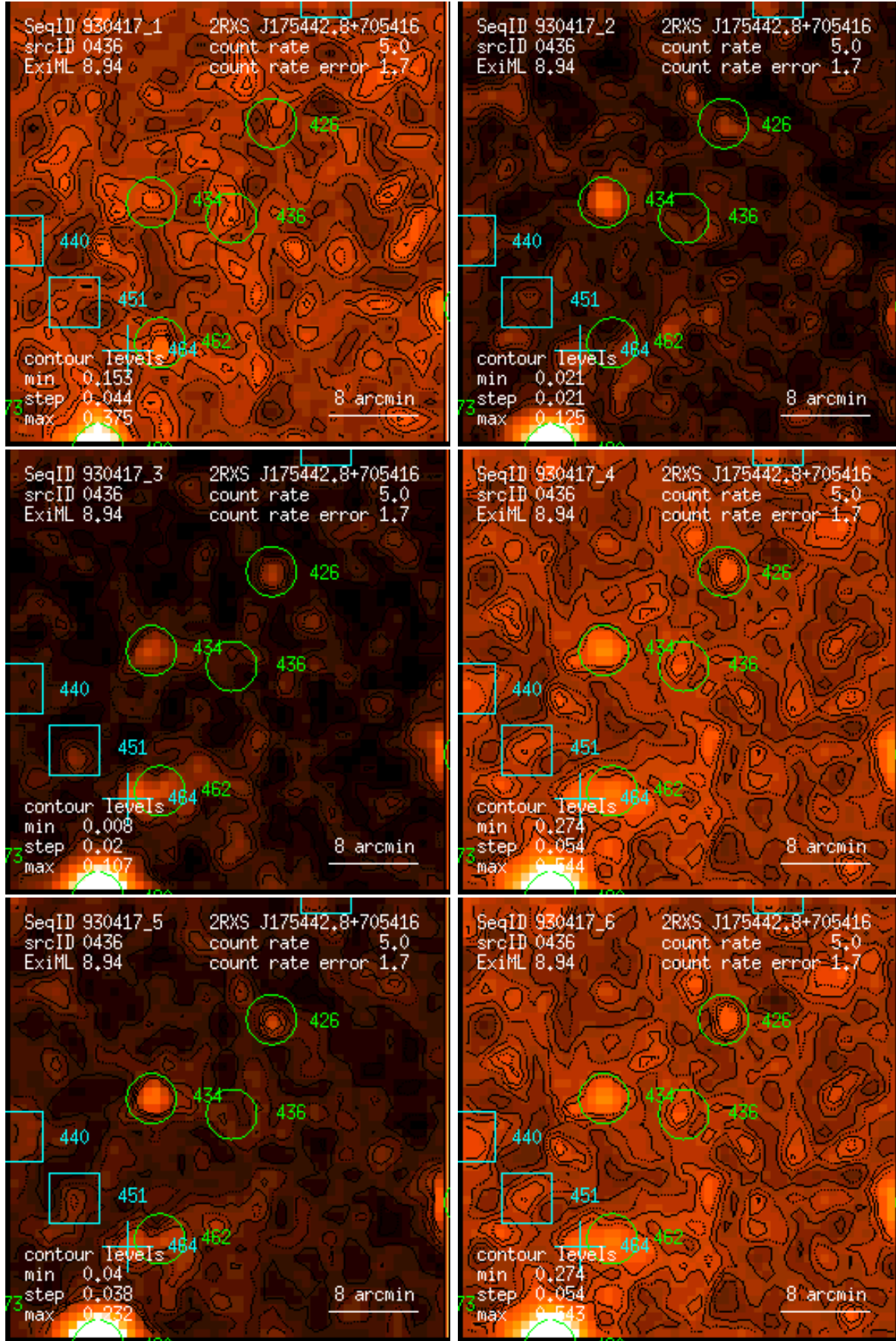
Figure 436: RASS 930417: detection 0436: band rate images, Gaussian filter: (1) PSPC channels 11 – 41, (2) 52 – 90, (3) 91 – 201, (4) 11 – 235, (5) 52 – 201, (6) 11 – 201. Broad band rates in counts/ks. Band rate contour levels in counts/ks/arcmin 2 .
