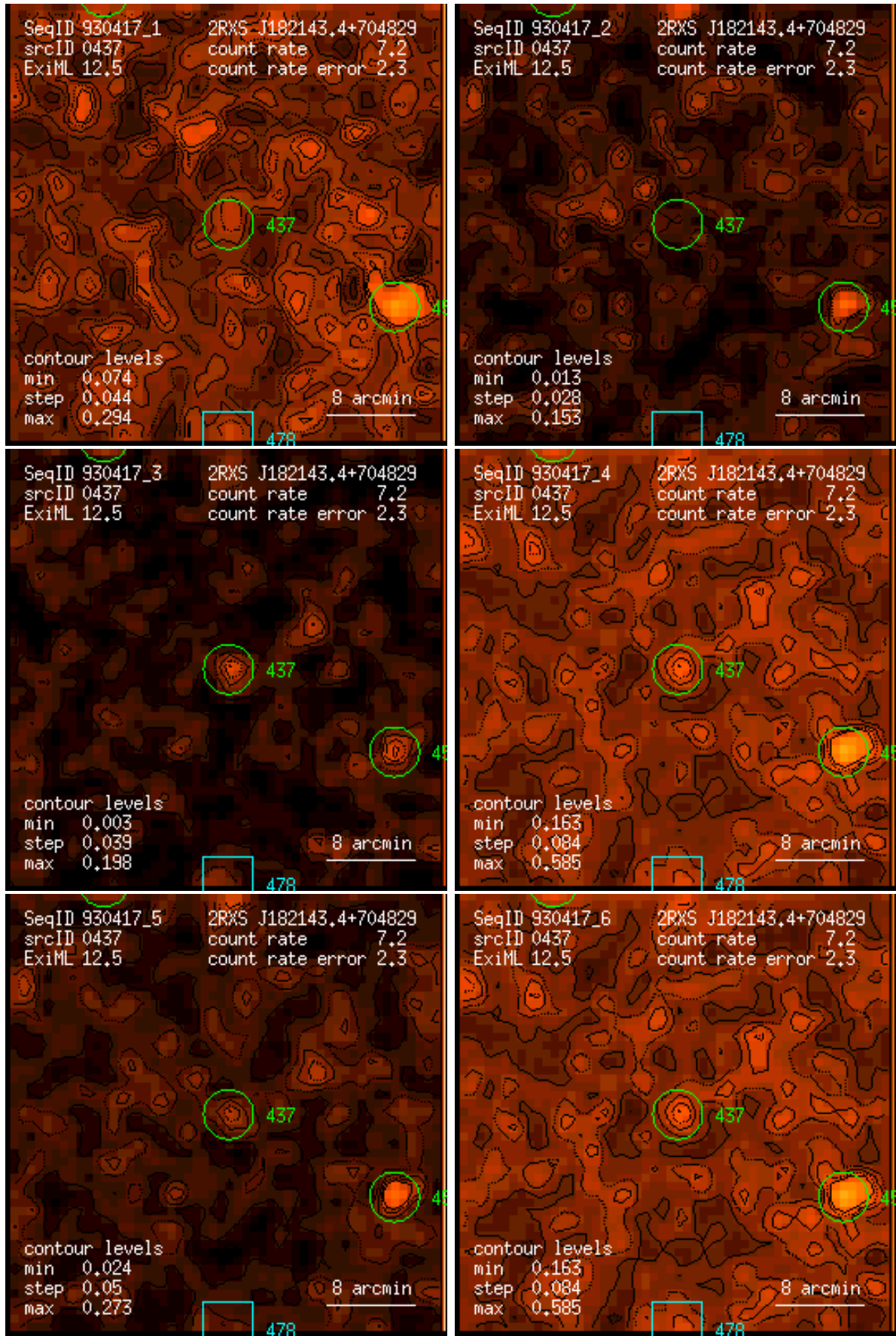
Figure 437: RASS 930417: detection 0437: band rate images, Gaussian filter: (1) PSPC channels 11 – 41, (2) 52 – 90, (3) 91 – 201, (4) 11 – 235, (5) 52 – 201, (6) 11 – 201. Broad band rates in counts/ks. Band rate contour levels in counts/ks/arcmin 2 .
