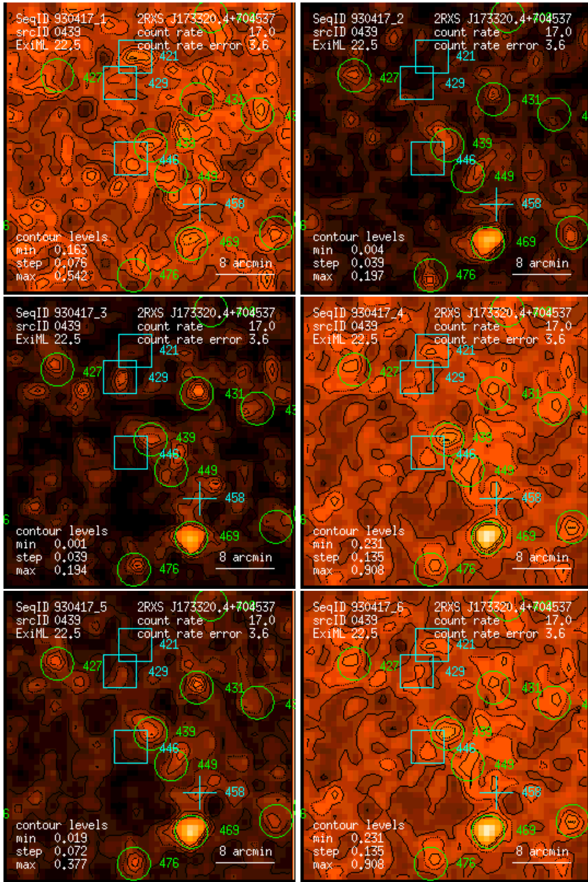
Figure 439: RASS 930417: detection 0439: band rate images, Gaussian filter: (1) PSPC channels 11 – 41, (2) 52 – 90, (3) 91 – 201, (4) 11 – 235, (5) 52 – 201, (6) 11 – 201. Broad band rates in counts/ks. Band rate contour levels in counts/ks/arcmin 2 .
