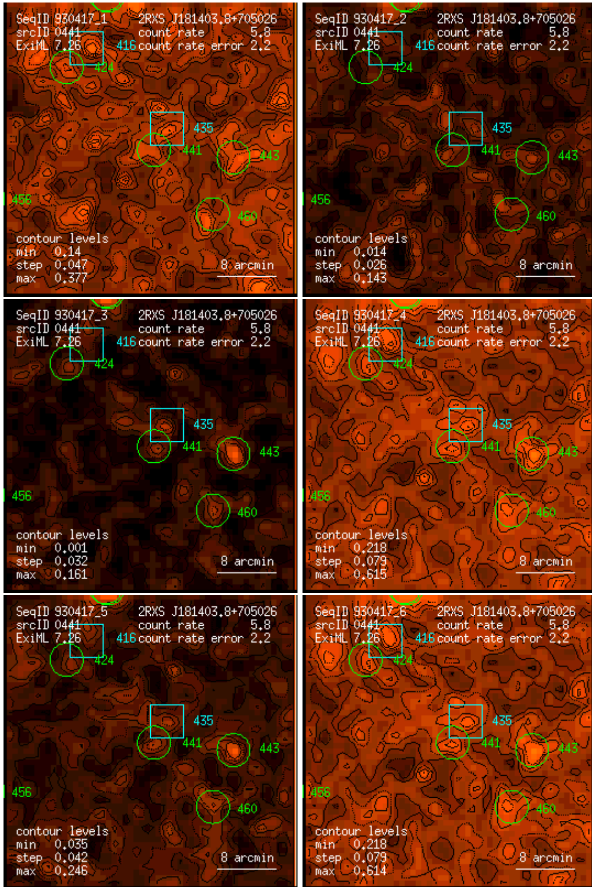
Figure 441: RASS 930417: detection 0441: band rate images, Gaussian filter: (1) PSPC channels 11 – 41, (2) 52 – 90, (3) 91 – 201, (4) 11 – 235, (5) 52 – 201, (6) 11 – 201. Broad band rates in counts/ks. Band rate contour levels in counts/ks/arcmin 2 .
