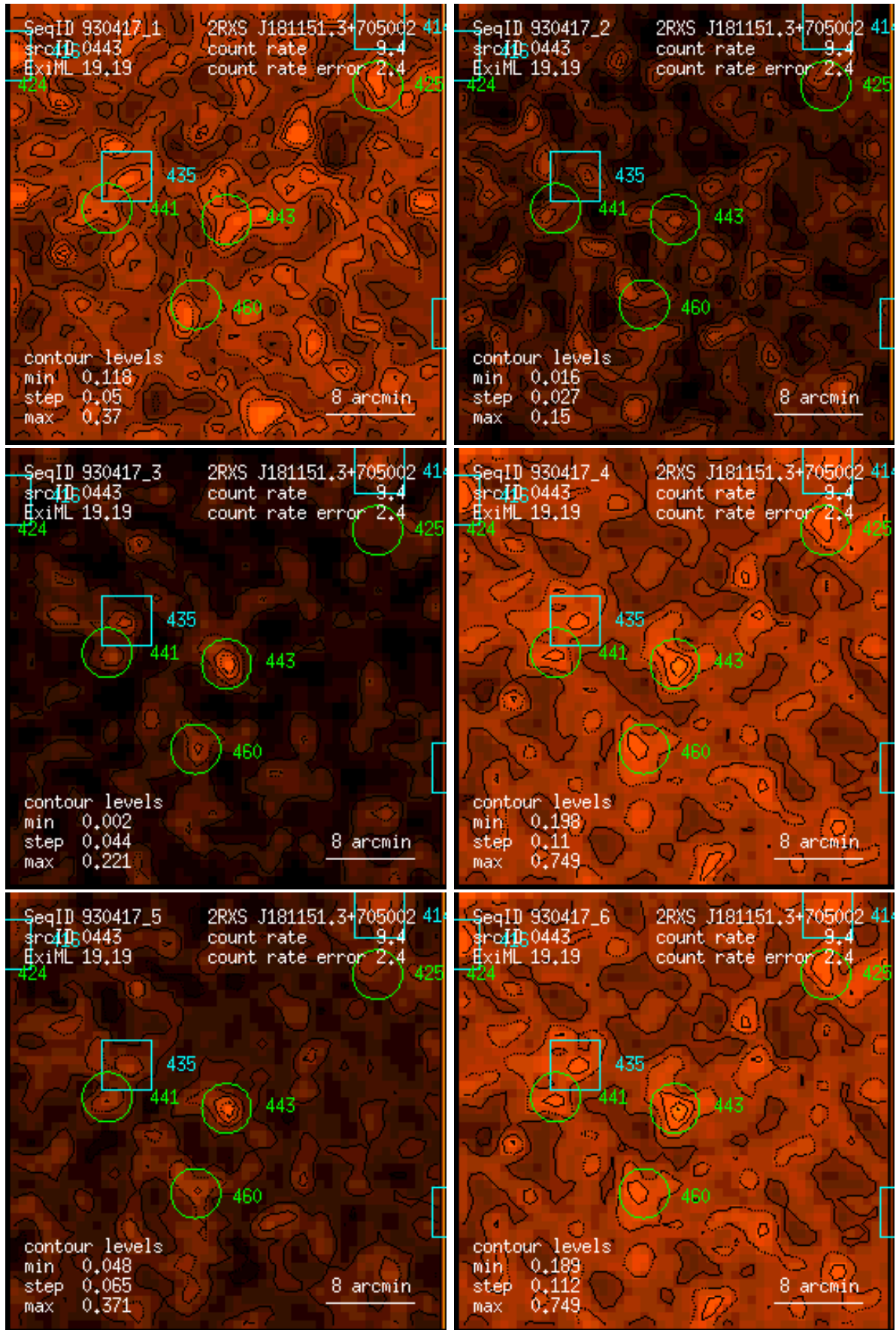
Figure 443: RASS 930417: detection 0443: band rate images, Gaussian filter: (1) PSPC channels 11 – 41, (2) 52 – 90, (3) 91 – 201, (4) 11 – 235, (5) 52 – 201, (6) 11 – 201. Broad band rates in counts/ks. Band rate contour levels in counts/ks/arcmin 2 .
