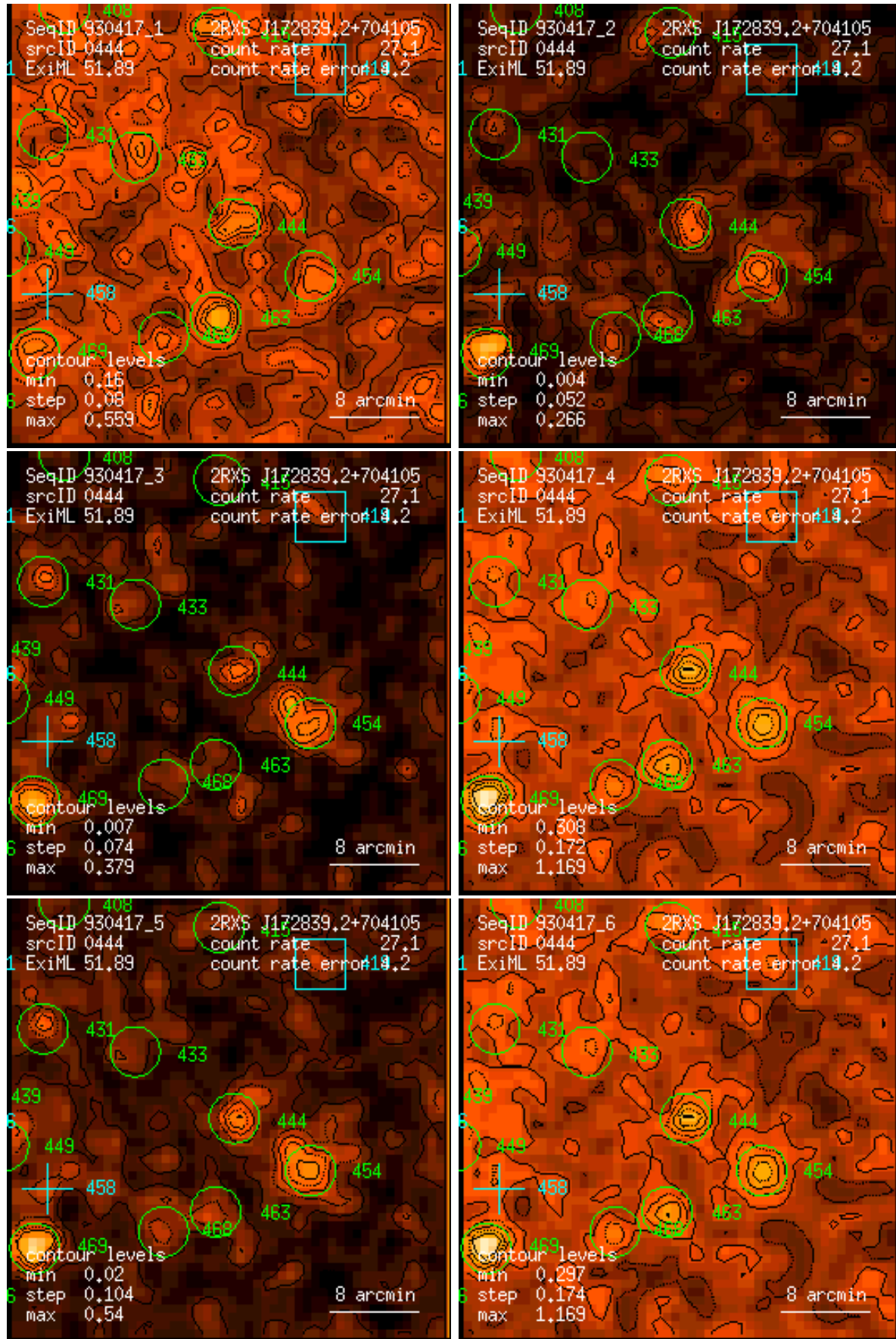
Figure 444: RASS 930417: detection 0444: band rate images, Gaussian filter: (1) PSPC channels 11 – 41, (2) 52 – 90, (3) 91 – 201, (4) 11 – 235, (5) 52 – 201, (6) 11 – 201. Broad band rates in counts/ks. Band rate contour levels in counts/ks/arcmin 2 .
