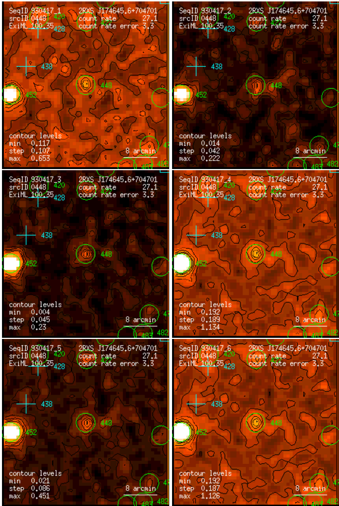
Figure 448: RASS 930417: detection 0448: band rate images, Gaussian filter: (1) PSPC channels 11 – 41, (2) 52 – 90, (3) 91 – 201, (4) 11 – 235, (5) 52 – 201, (6) 11 – 201. Broad band rates in counts/ks. Band rate contour levels in counts/ks/arcmin 2 .
