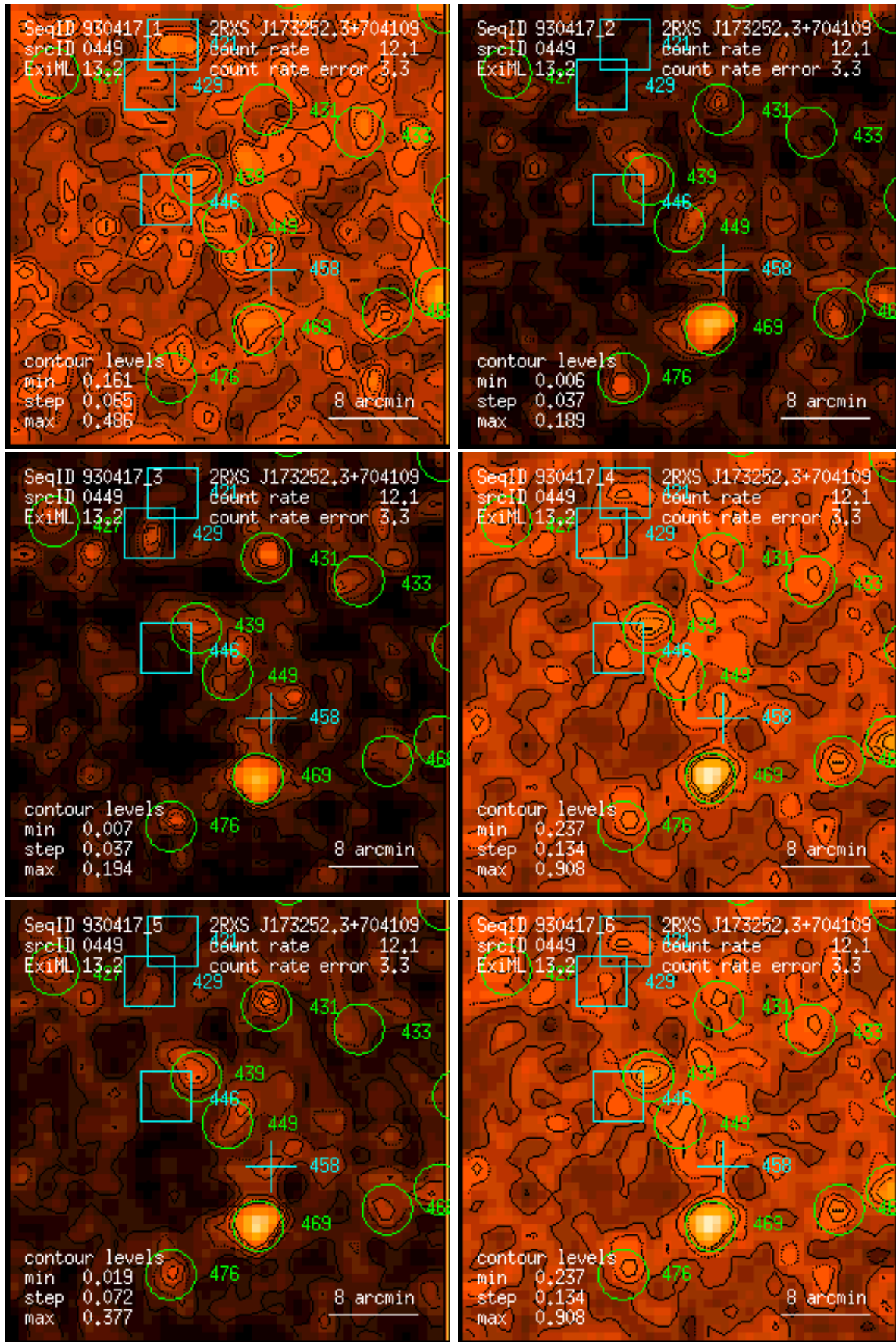
Figure 449: RASS 930417: detection 0449: band rate images, Gaussian filter: (1) PSPC channels 11 – 41, (2) 52 – 90, (3) 91 – 201, (4) 11 – 235, (5) 52 – 201, (6) 11 – 201. Broad band rates in counts/ks. Band rate contour levels in counts/ks/arcmin 2 .
