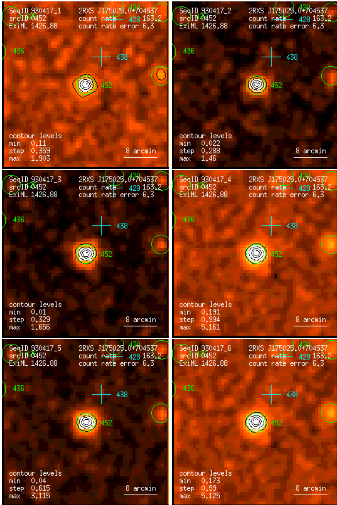
Figure 452: RASS 930417: detection 0452: band rate images, Gaussian filter: (1) PSPC channels 11 – 41, (2) 52 – 90, (3) 91 – 201, (4) 11 – 235, (5) 52 – 201, (6) 11 – 201. Broad band rates in counts/ks. Band rate contour levels in counts/ks/arcmin 2 .
